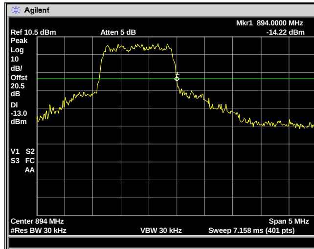
Figure 28: Band-Edge CDMA High Channel
