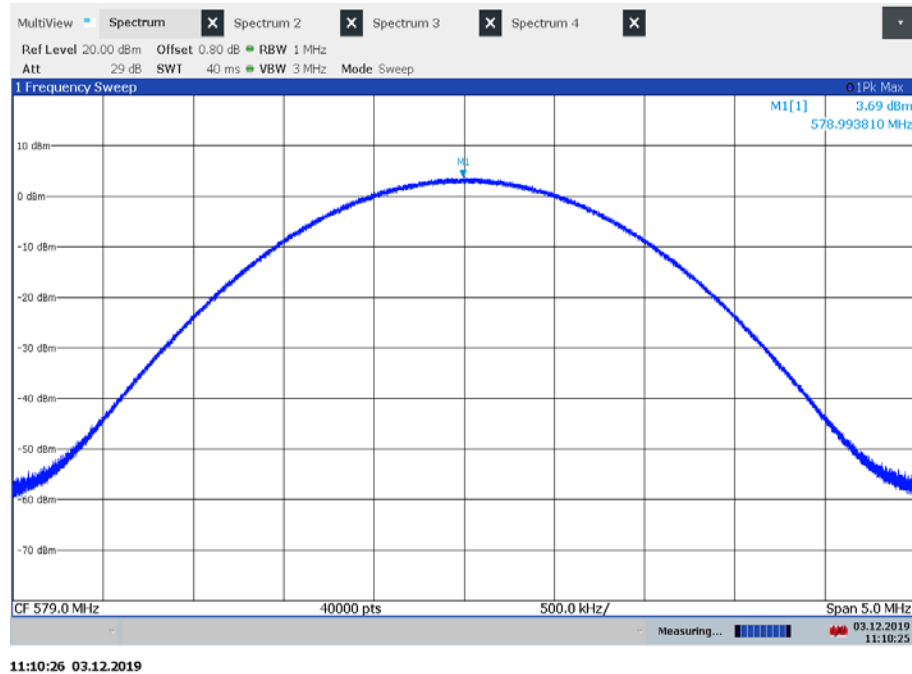
Plot 3: middle channel, conducted peak power
