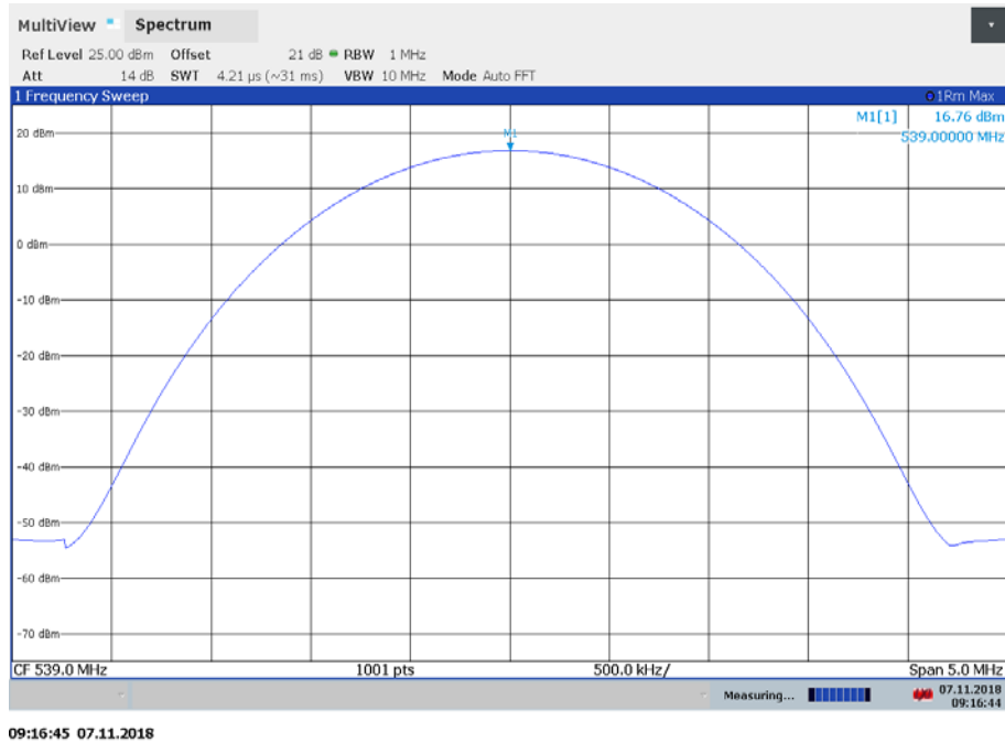
Plot 1: middle channel, average (modulated carrier)
