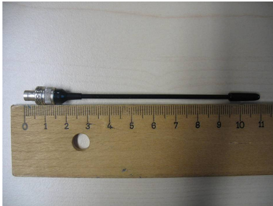
Photo 10: (L)-Type / Antenna 2
