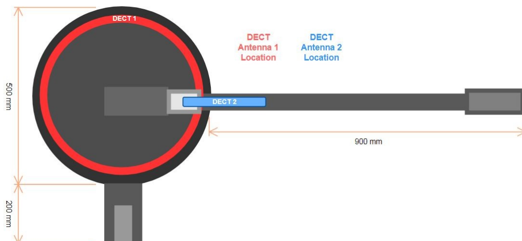
Fig. 1: Sketches and antenna locations of the EUT (marked in red and blue).
