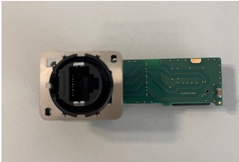
Bottom View (RJ45 PCB)
