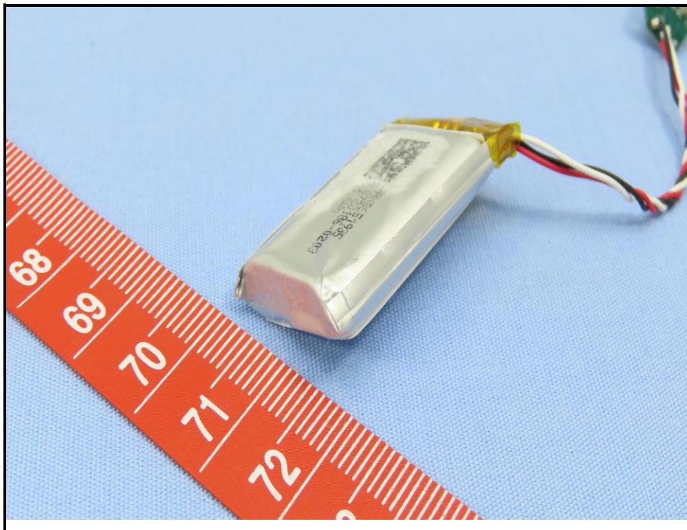
Charging Case (Second battery cell)
