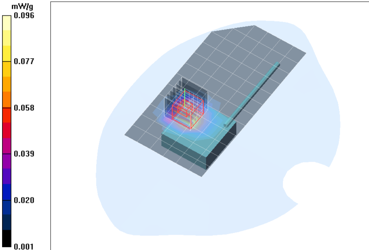
Fig. 1: SAR distribution for Sennheiser Communications DW 20 HS, head configuration below the flat part of SAM phantom, test position 1, antenna 1, mid channel.
