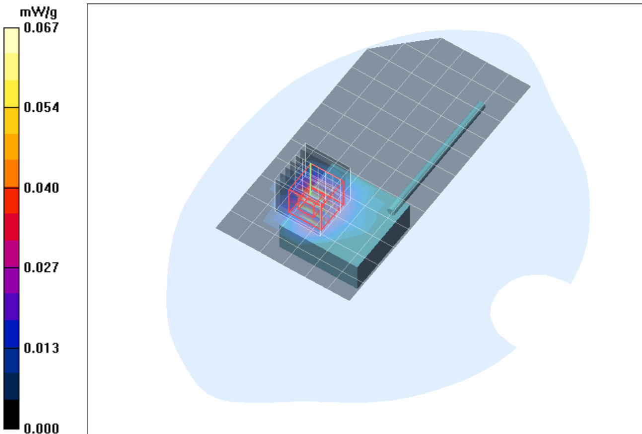
Fig. 2: SAR distribution for Sennheiser Communications DW 20 HS, head configuration below the flat part of SAM phantom, test position 1, antenna 2, mid channel.
