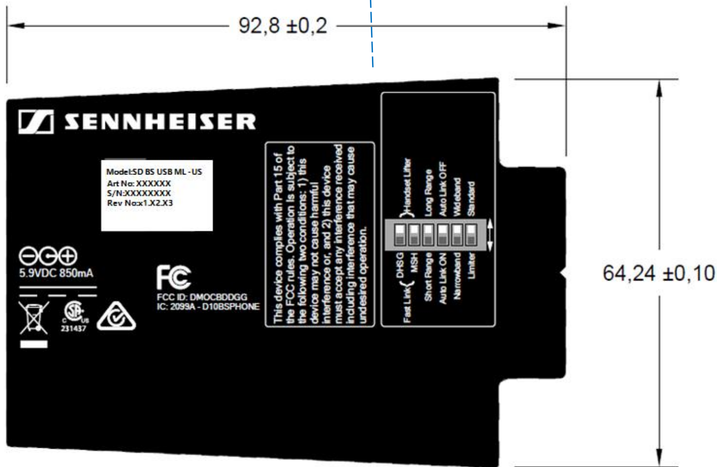
Figure 1.1: SD BS USB ML -US (view from back)
