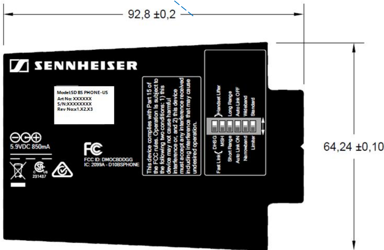
Figure 1.1: SD BS PHONE -US (view from back)
