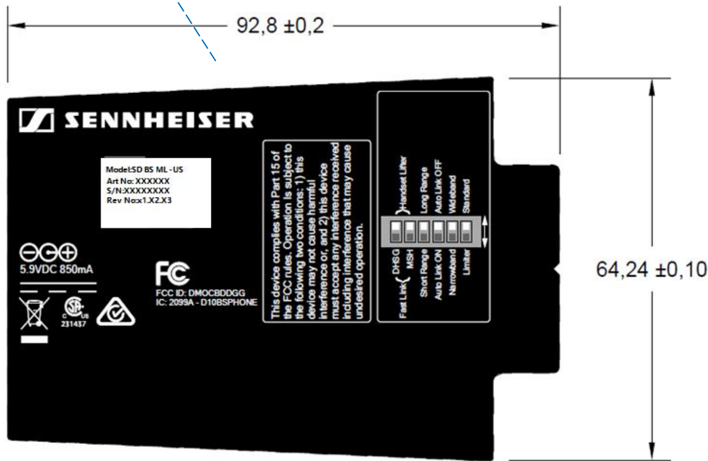
Figure 1.1: SD BS ML -US (view from back)
