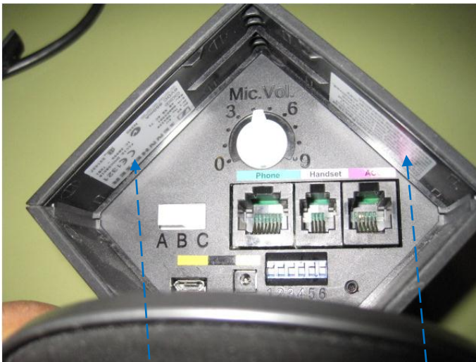
Figure 1.1 : Position of the labels on the back side of OR BS –US base
