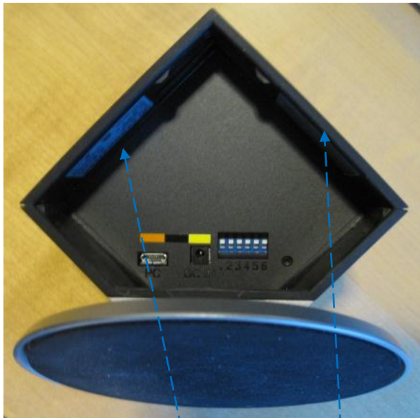
Figure 1.1: Labels position on the DW BS USB -US /Back view:
