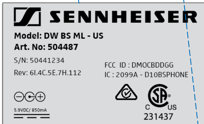
Figure 1.1: Position of the labels on the on the DW BS ML-US /back view
