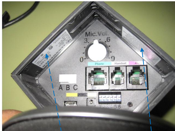
Figure 1.1: Position of the labels on the on the DW BS ML-US /back view
