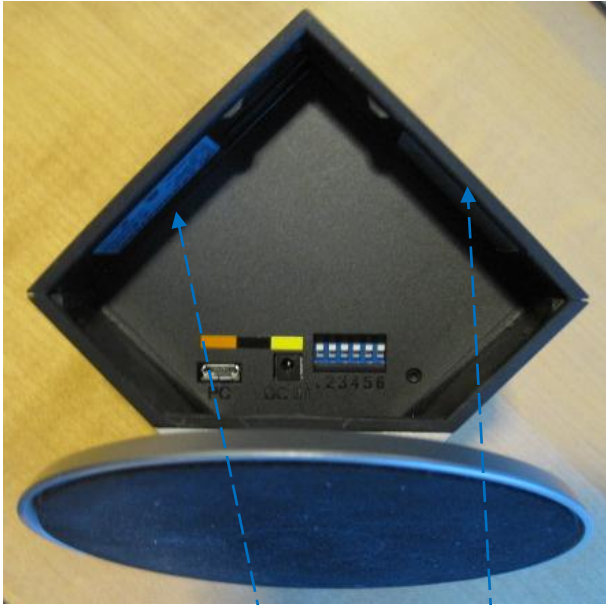
Figure 1.1: Labels position on the DW BS USB ML -US /Back view:
