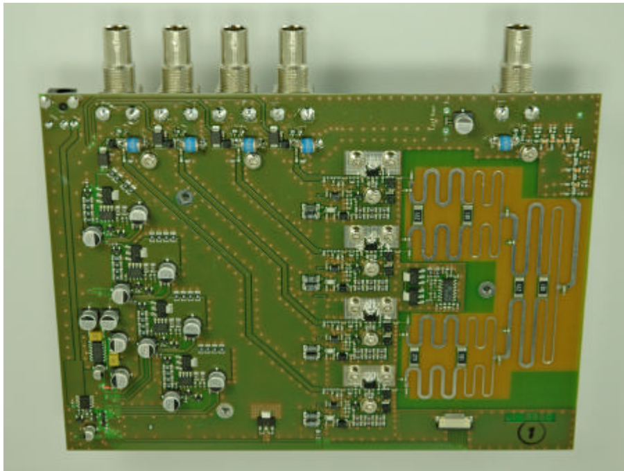
Mainboard
