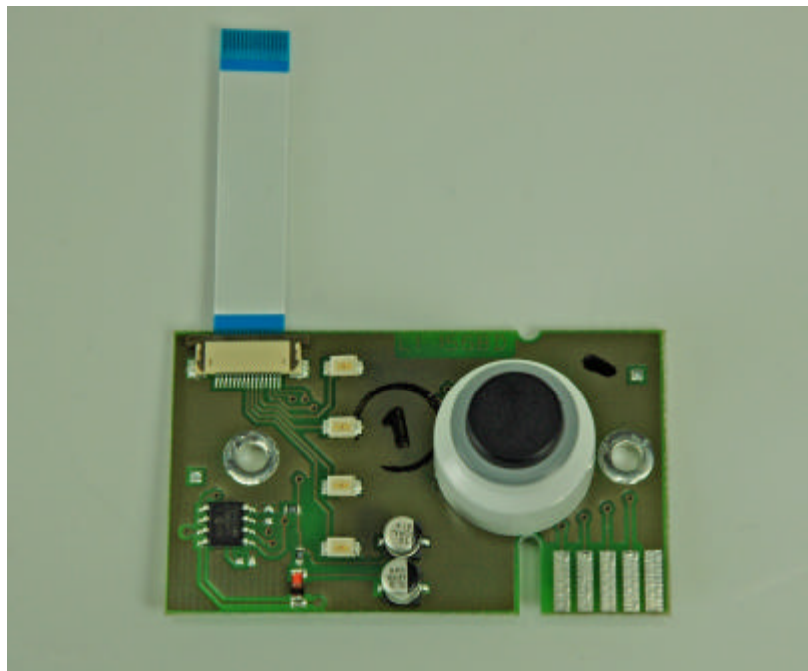
Controlboard
