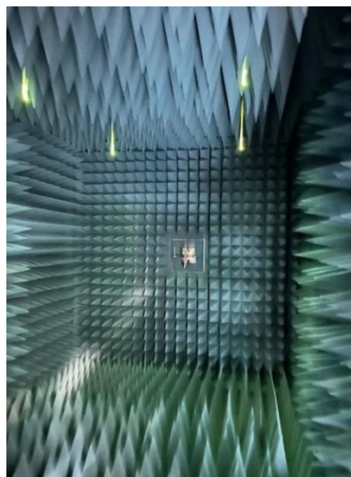
Figure 8 – Photo of Shure Antenna Test Chamber.
