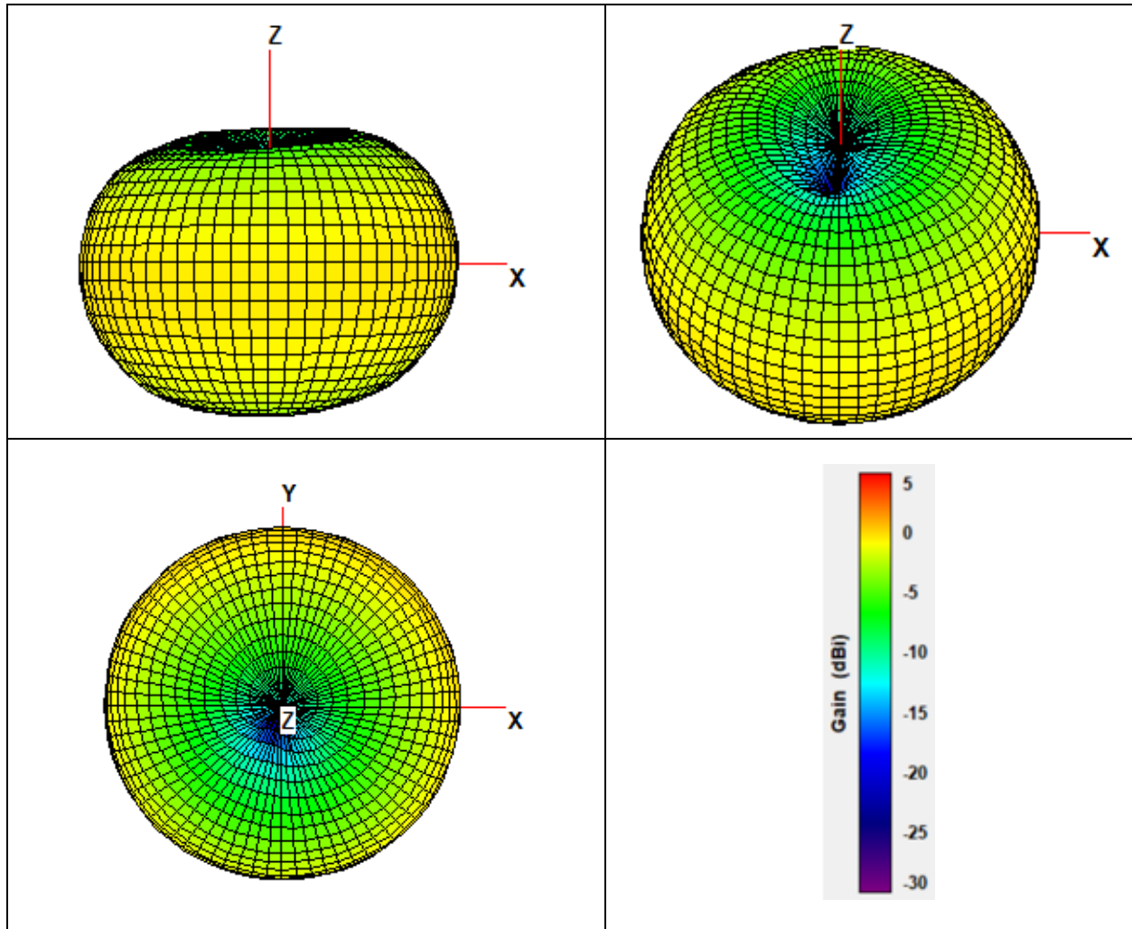
Figure 5 – SLXD1+ G57-variant (580.000 MHz) 3D radiation patterns and scale
