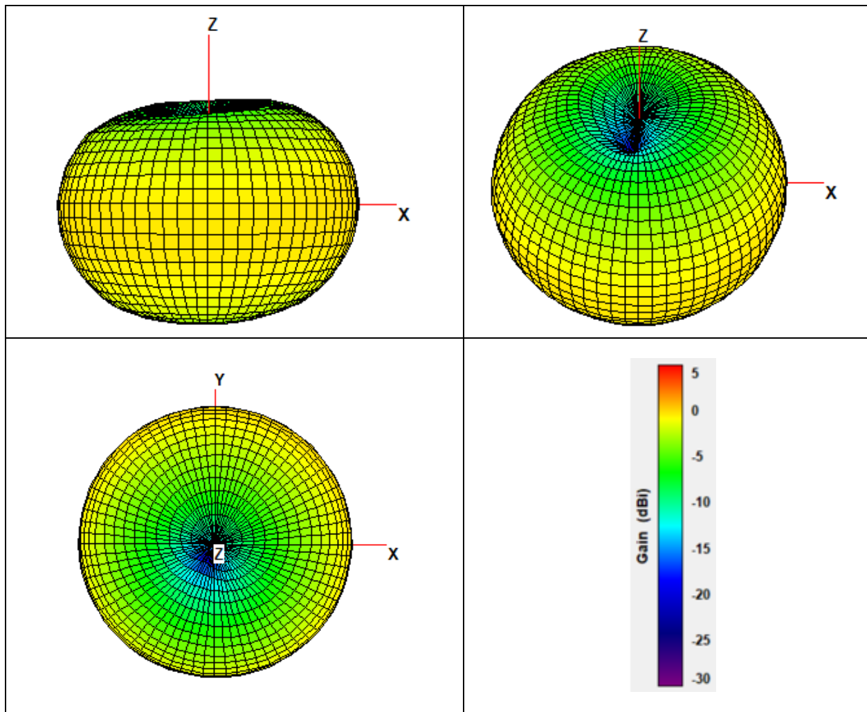
Figure 6 – SLXD1+ G57-variant (607.875 MHz) 3D radiation patterns and scale
