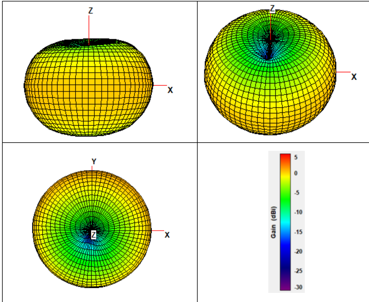
Figure 4 – SLXD1+ G57-variant (552.150 MHz) 3D radiation patterns and scale
