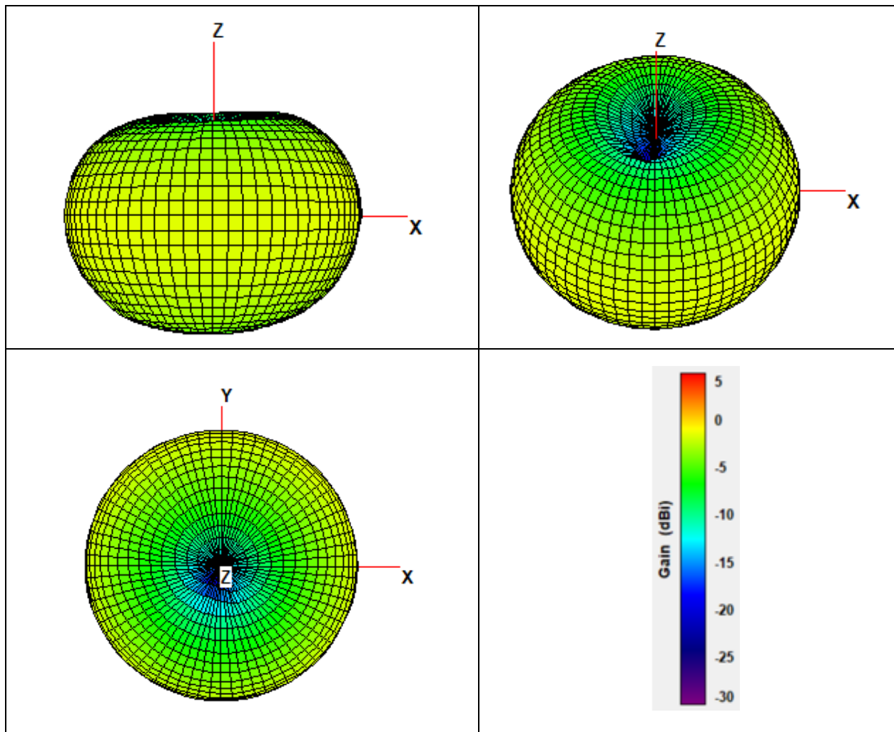
Figure 2 – SLXD1+ G57-variant (510.000 MHz) 3D radiation patterns and scale
