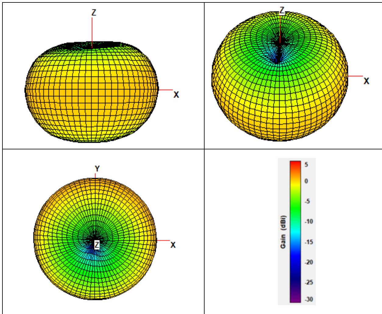
Figure 3 – SLXD1+ G57-variant (551.850 MHz) 3D radiation patterns and scale
