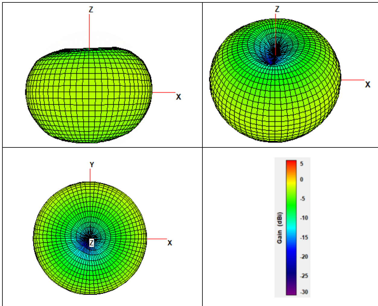
Figure 1 – SLXD1+ G57-variant (470.125 MHz) 3D radiation patterns and scale
