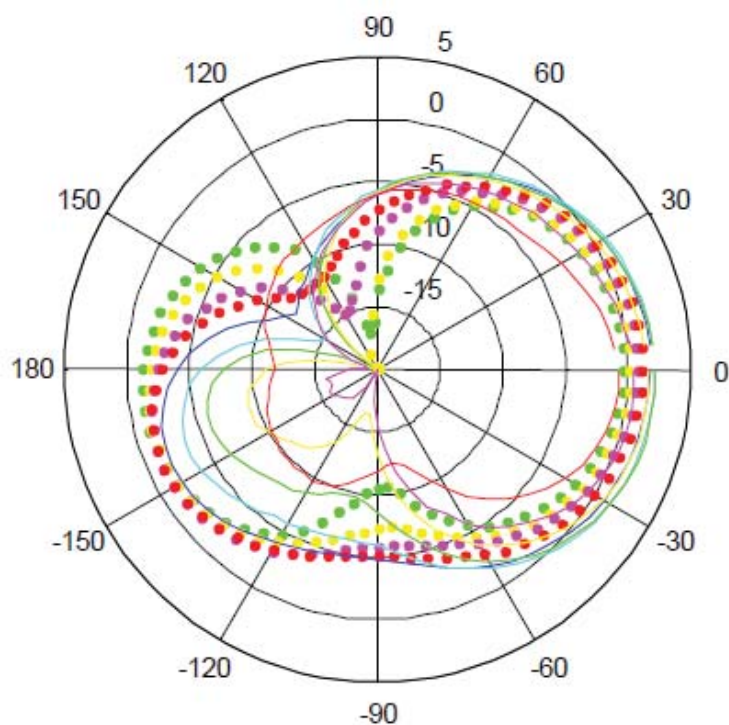
Figure 1 - PIFA in single configuration at 1.9 GHz
