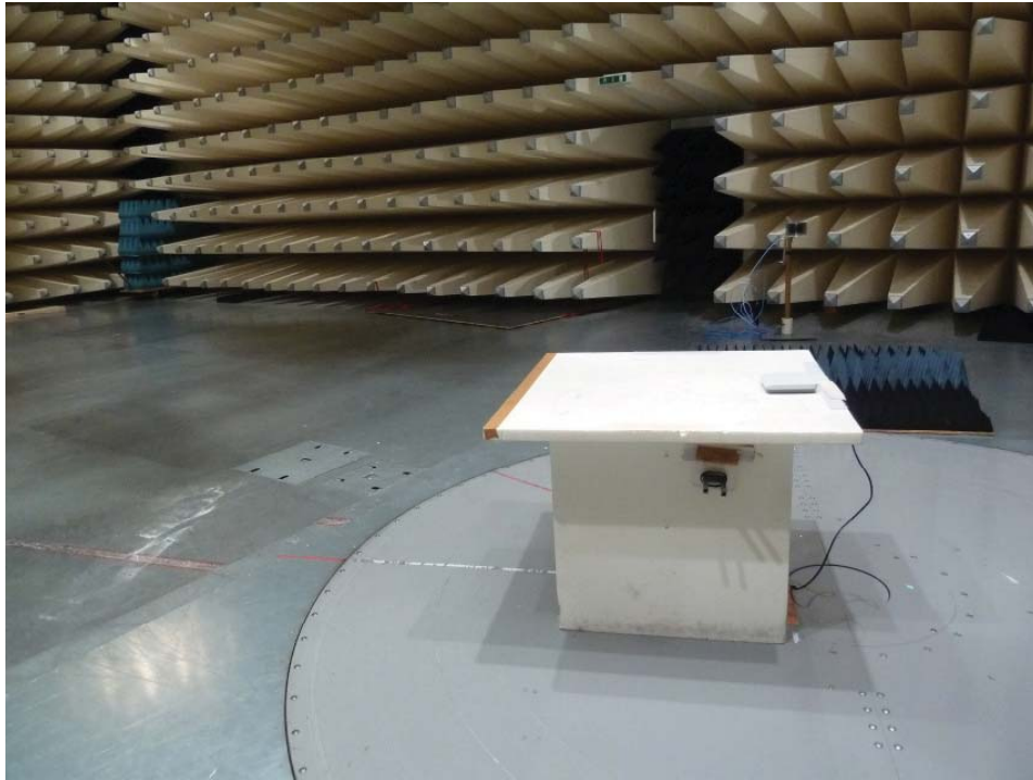
Photo 3: Radiated Emission
