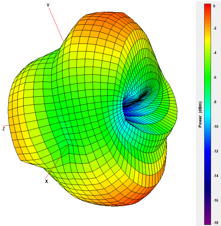
Figure 3-4. 1.9GHz Antenna B 3D
