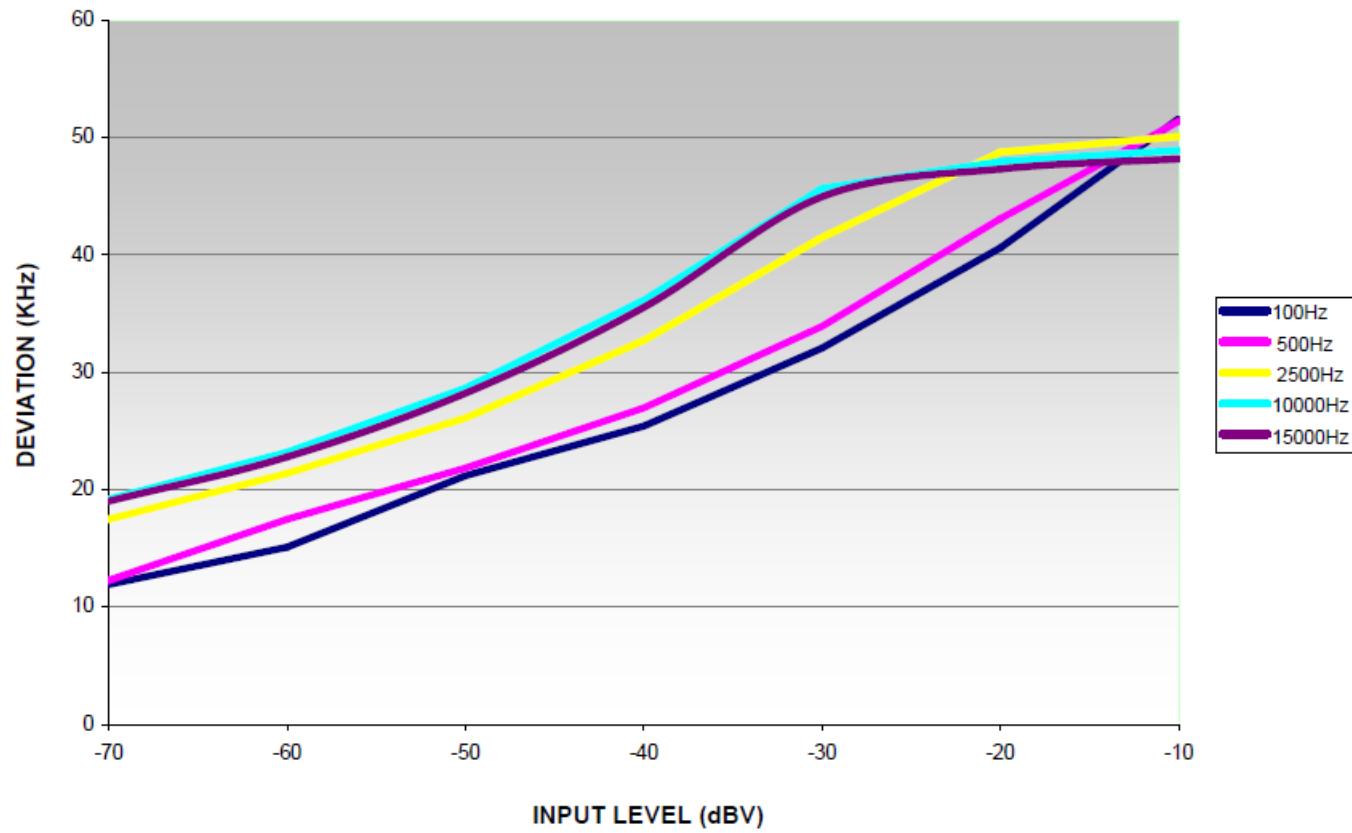
MX690 DEVIATION vs. INPUT LEVEL
