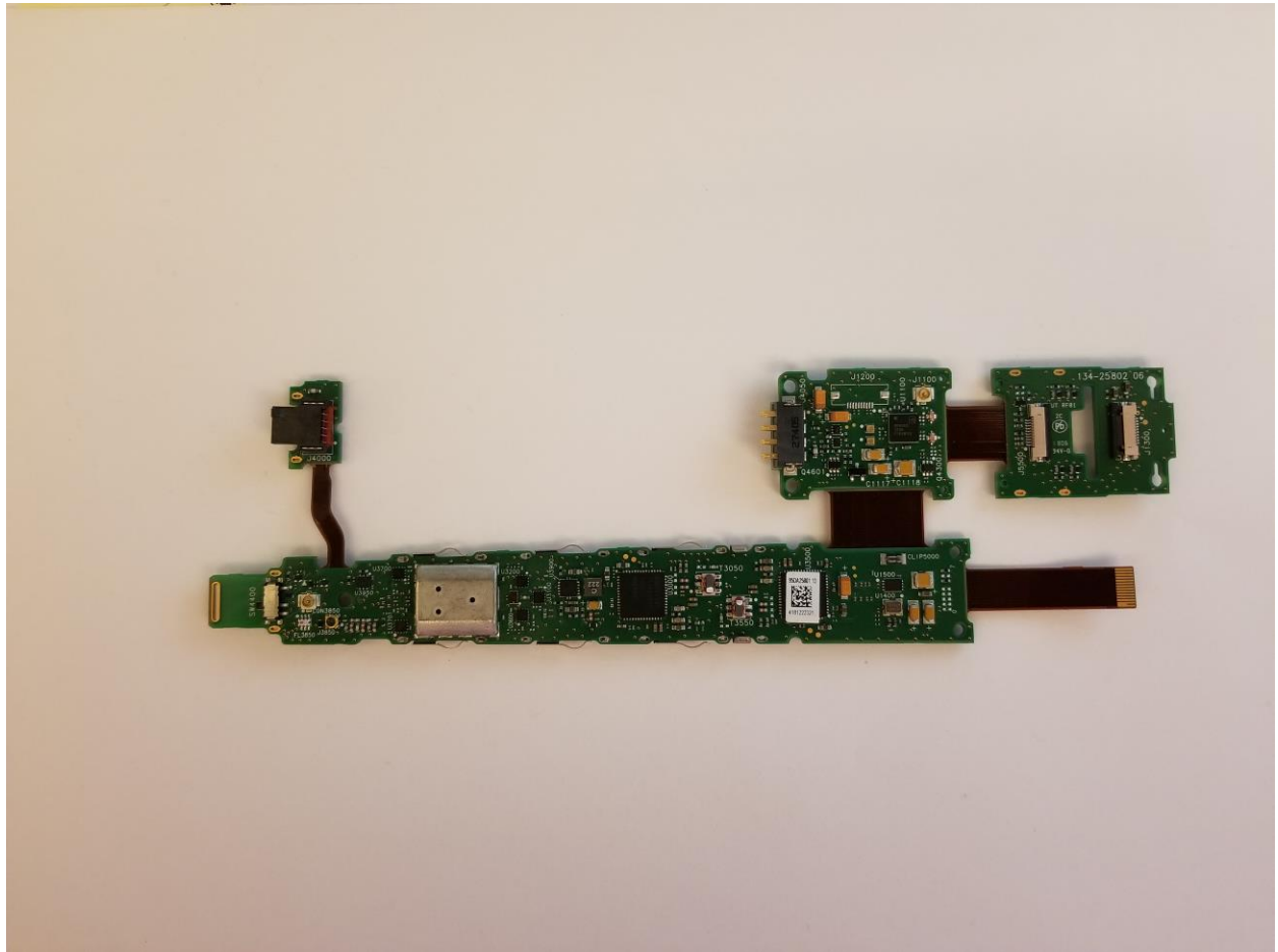
ADX2FD Circuit Board Top (with shields in place)
