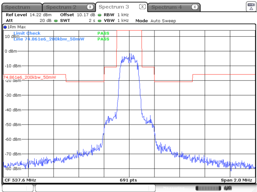
D2 mode: 537.600 MHz, Emission Mask (2)
