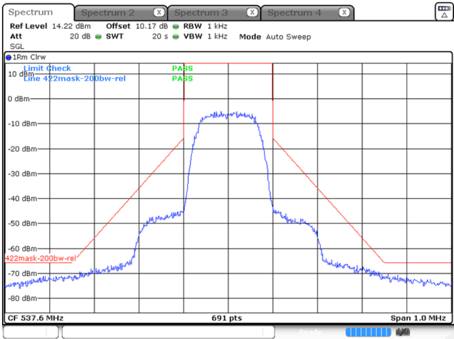
D2 mode: 537.600 MHz, Emission Mask (1)
