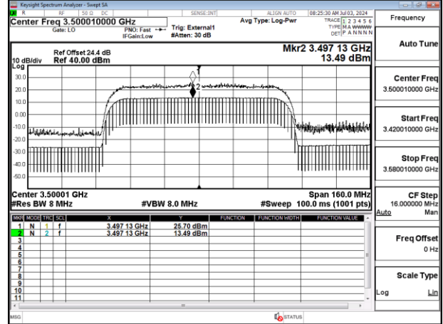
Band77-Part27_80MHz_CP_OFDM_SCS30kHz_256QAM_RB217_0_Chain1_CH633334
