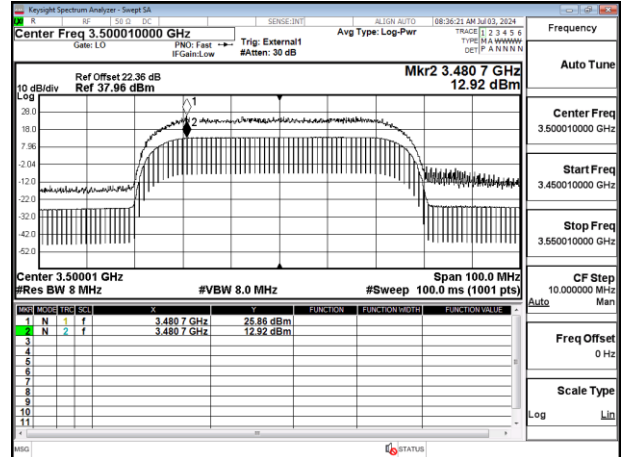
Band77-Part27_50MHz_CP_OFDM_SCS30kHz_256QAM_RB133_0_Chain1_CH633334
