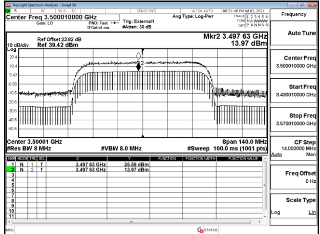
Band77-Part27_70MHz_CP_OFDM_SCS30kHz_256QAM_RB189_0_Chain0_CH633334
