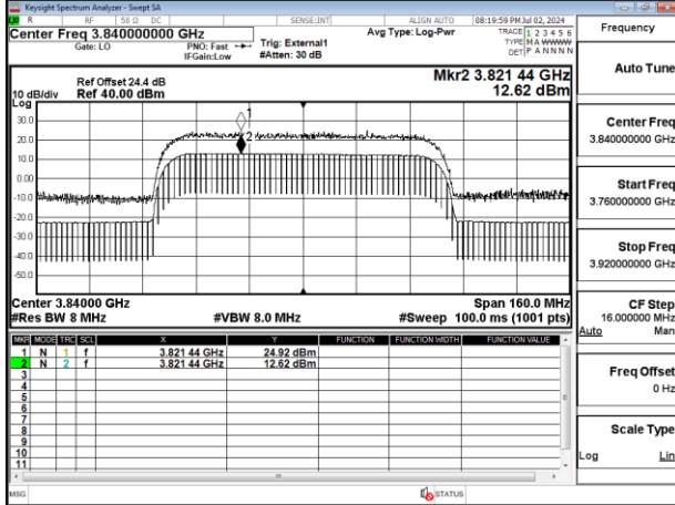
Band77-Part27_80MHz_CP_OFDM_SCS30kHz_256QAM_RB217_0_Chain0_CH656000
