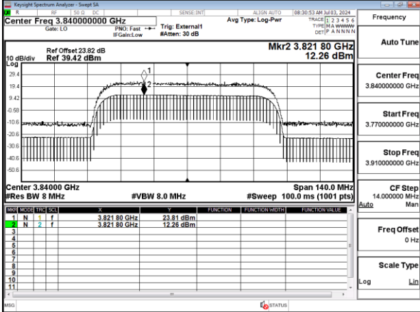
Band77-Part27_70MHz_CP_OFDM_SCS30kHz_256QAM_RB189_0_Chain1_CH656000
