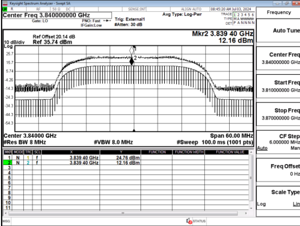
Band77-Part27_30MHz_CP_OFDM_SCS30kHz_256QAM_RB78_0_Chain1_CH656000
