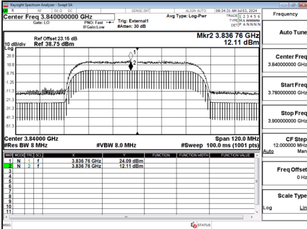
Band77-Part27_60MHz_CP_OFDM_SCS30kHz_256QAM_RB162_0_Chain1_CH656000
