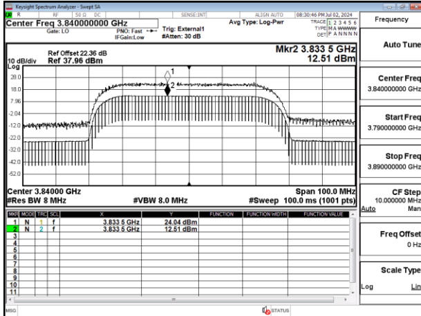
Band77-Part27_50MHz_CP_OFDM_SCS30kHz_256QAM_RB133_0_Chain0_CH656000
