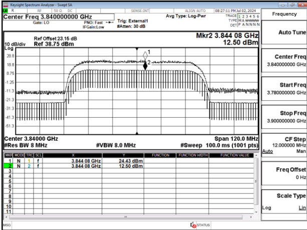
Band77-Part27_60MHz_CP_OFDM_SCS30kHz_256QAM_RB162_0_Chain0_CH656000
