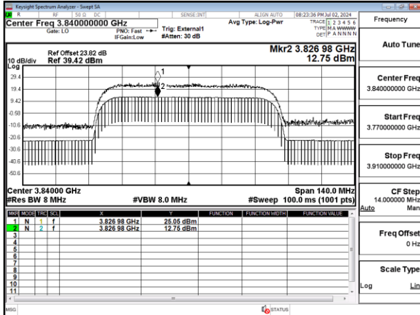
Band77-Part27_70MHz_CP_OFDM_SCS30kHz_256QAM_RB189_0_Chain0_CH656000
