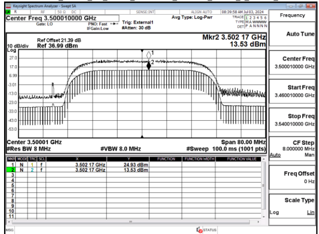
Band77-Part27_40MHz_CP_OFDM_SCS30kHz_256QAM_RB106_0_Chain1_CH633334
