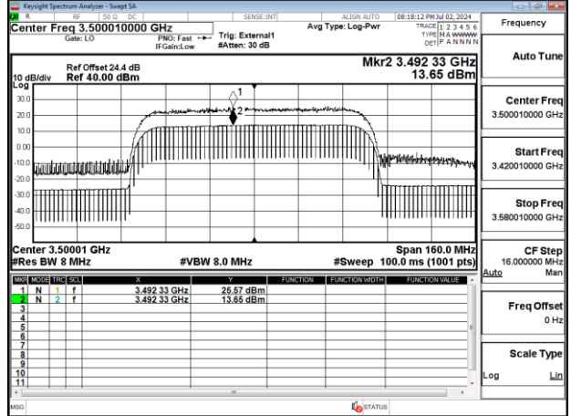
Band77-Part27_80MHz_CP_OFDM_SCS30kHz_256QAM_RB217_0_Chain0_CH633334
