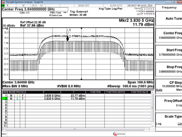
Band77-Part27_50MHz_CP_OFDM_SCS30kHz_256QAM_RB133_0_Chain1_CH656000
