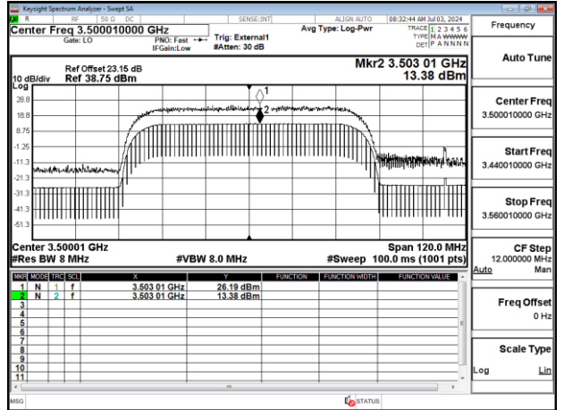
Band77-Part27_60MHz_CP_OFDM_SCS30kHz_256QAM_RB162_0_Chain1_CH633334
