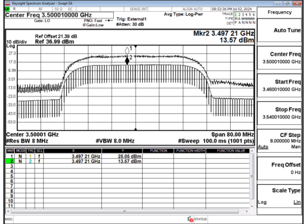
Band77-Part27_40MHz_CP_OFDM_SCS30kHz_256QAM_RB106_0_Chain0_CH633334
