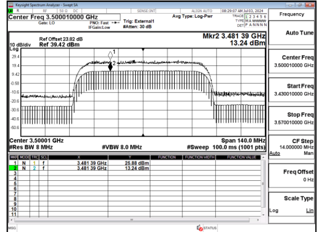
Band77-Part27_70MHz_CP_OFDM_SCS30kHz_256QAM_RB189_0_Chain1_CH633334
