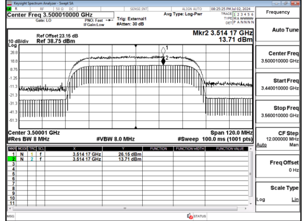
Band77-Part27_60MHz_CP_OFDM_SCS30kHz_256QAM_RB162_0_Chain0_CH633334
