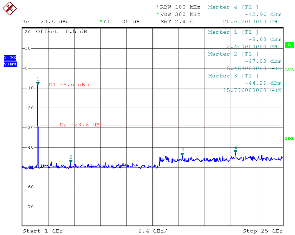
(Plot 2.4 C.2: Channel = 11, 1GHz to 25GHz@ 802.11b)
