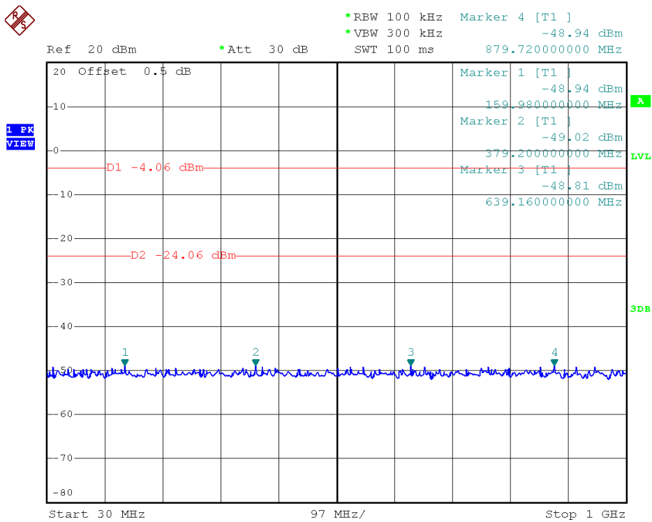
(Plot 2.4 I.1: Channel = 11, 30MHz to 1GHz@ 802.11n-20)
