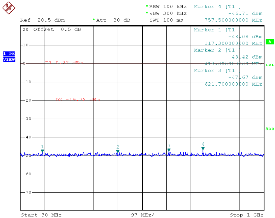
(Plot 2.4 G.1: Channel = 1, 30MHz to 1GHz@ 802.11n-20)
