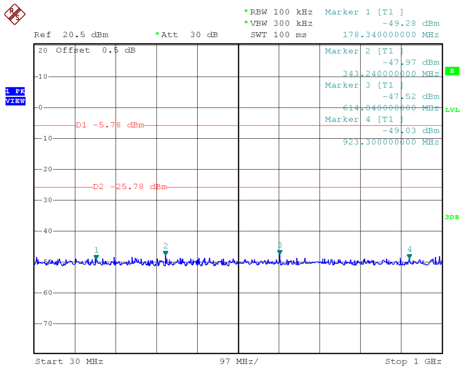
(Plot 2.4 A.1: Channel = 1, 30MHz to 1GHz@ 802.11b)
