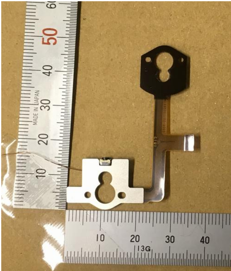
FPC COMMAND_B
