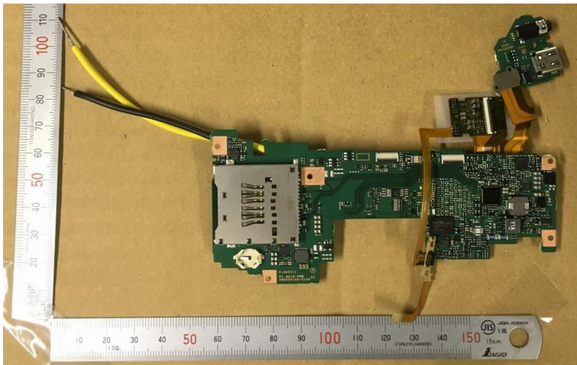
PWB MAIN_A
