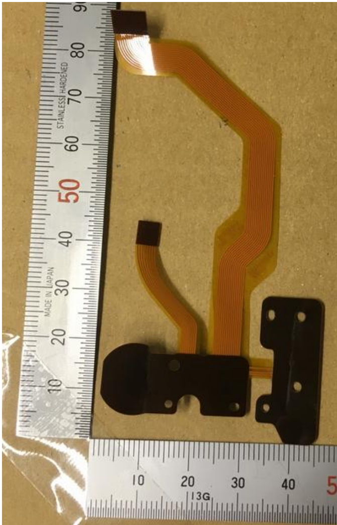
FPC REAR JOG_B
