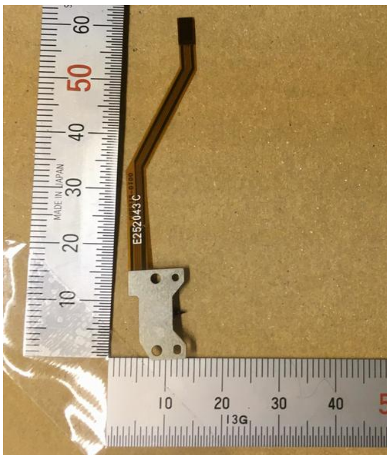
FPC AF_B
