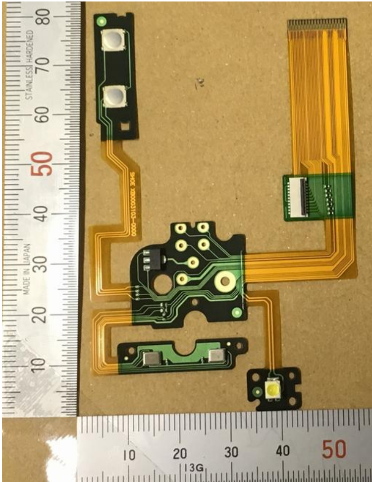
FPC SHOE_B
