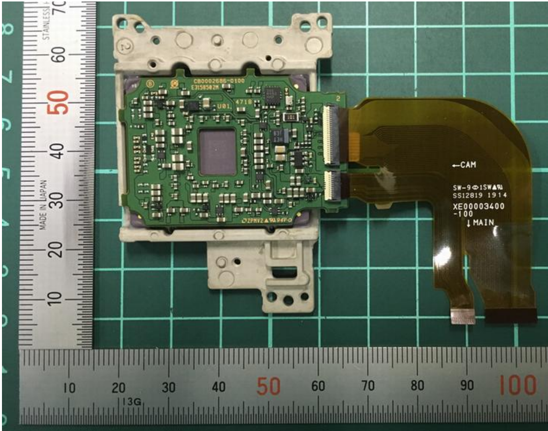
PWB CMOS_B
