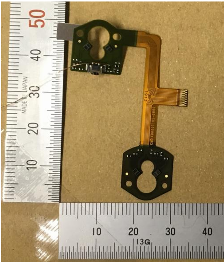
FPC COMMAND_B
