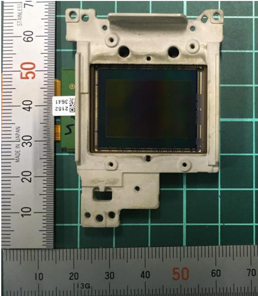
PWB CMOS_B
