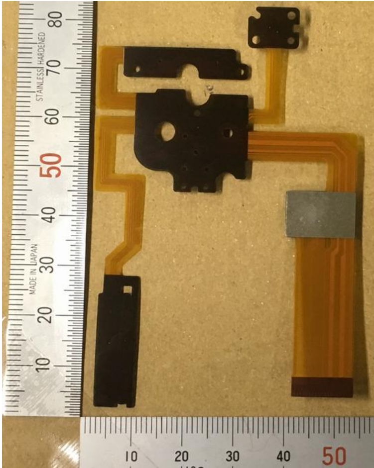
FPC SHOE_B
