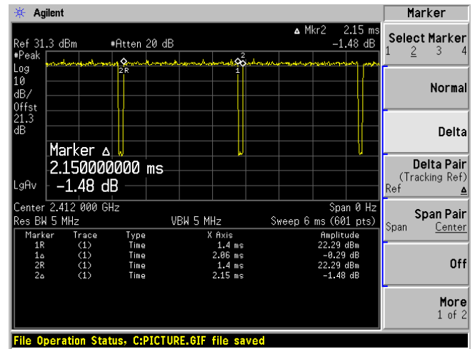
802.11g mode
