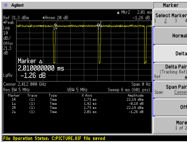
802.11n20 mode
