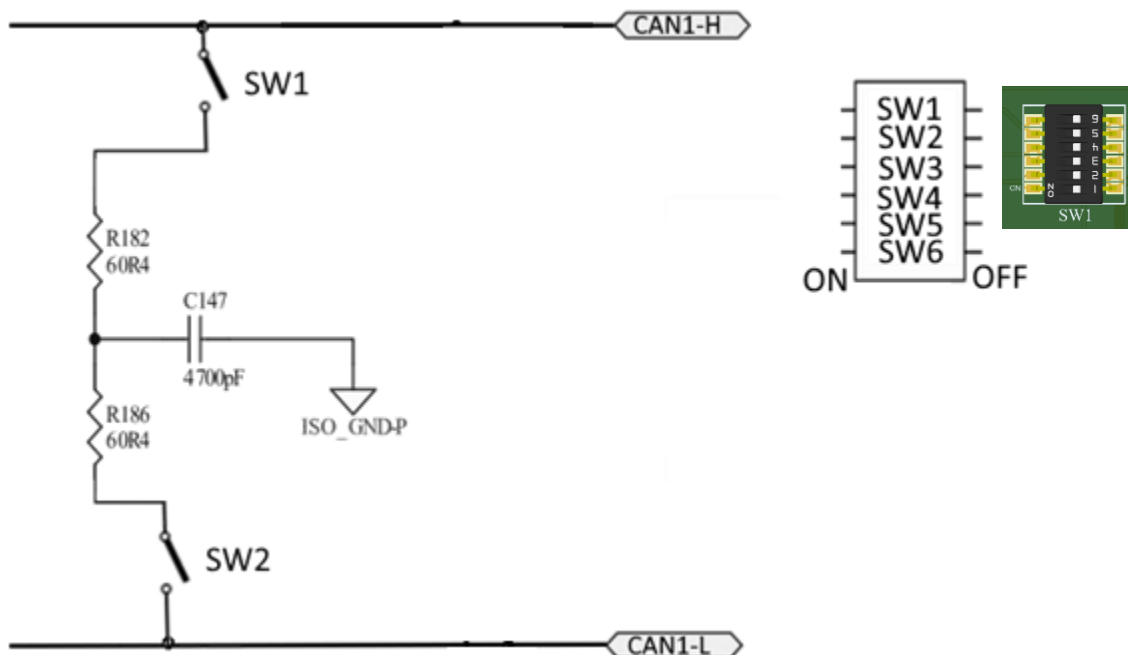
Figure 7 CAN Terminations
