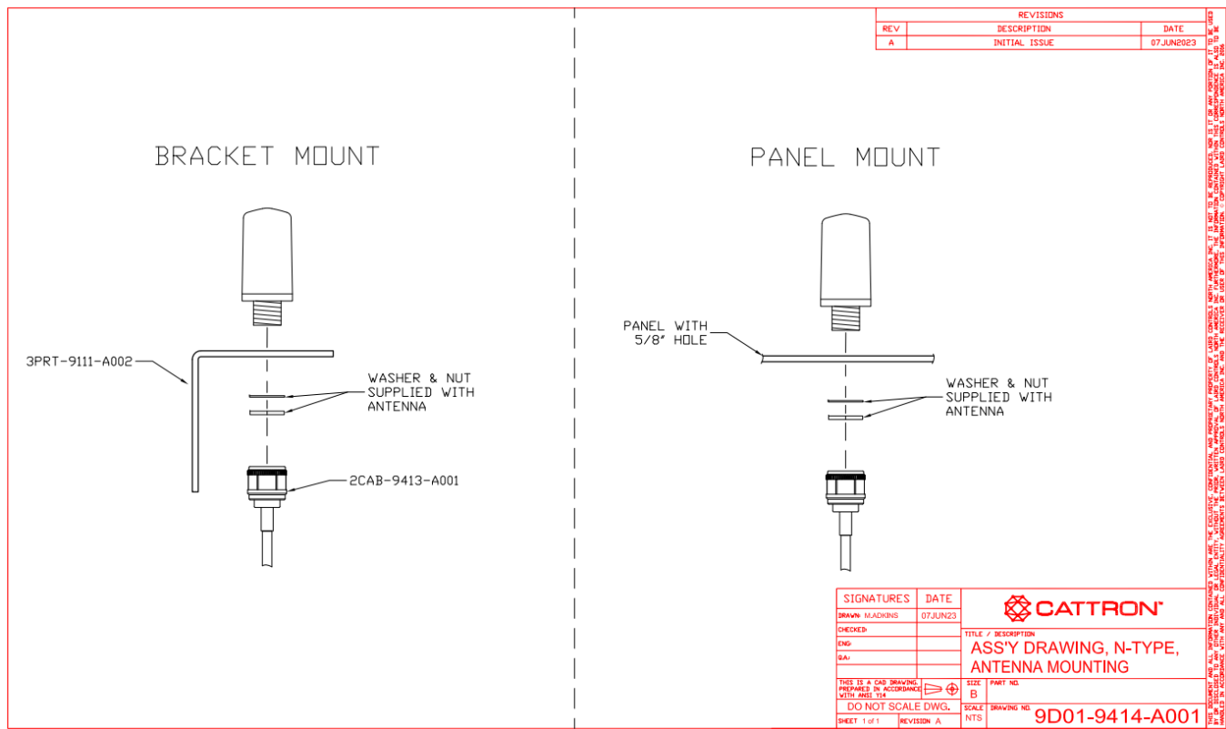
Figure 4 Antenna Mounting
