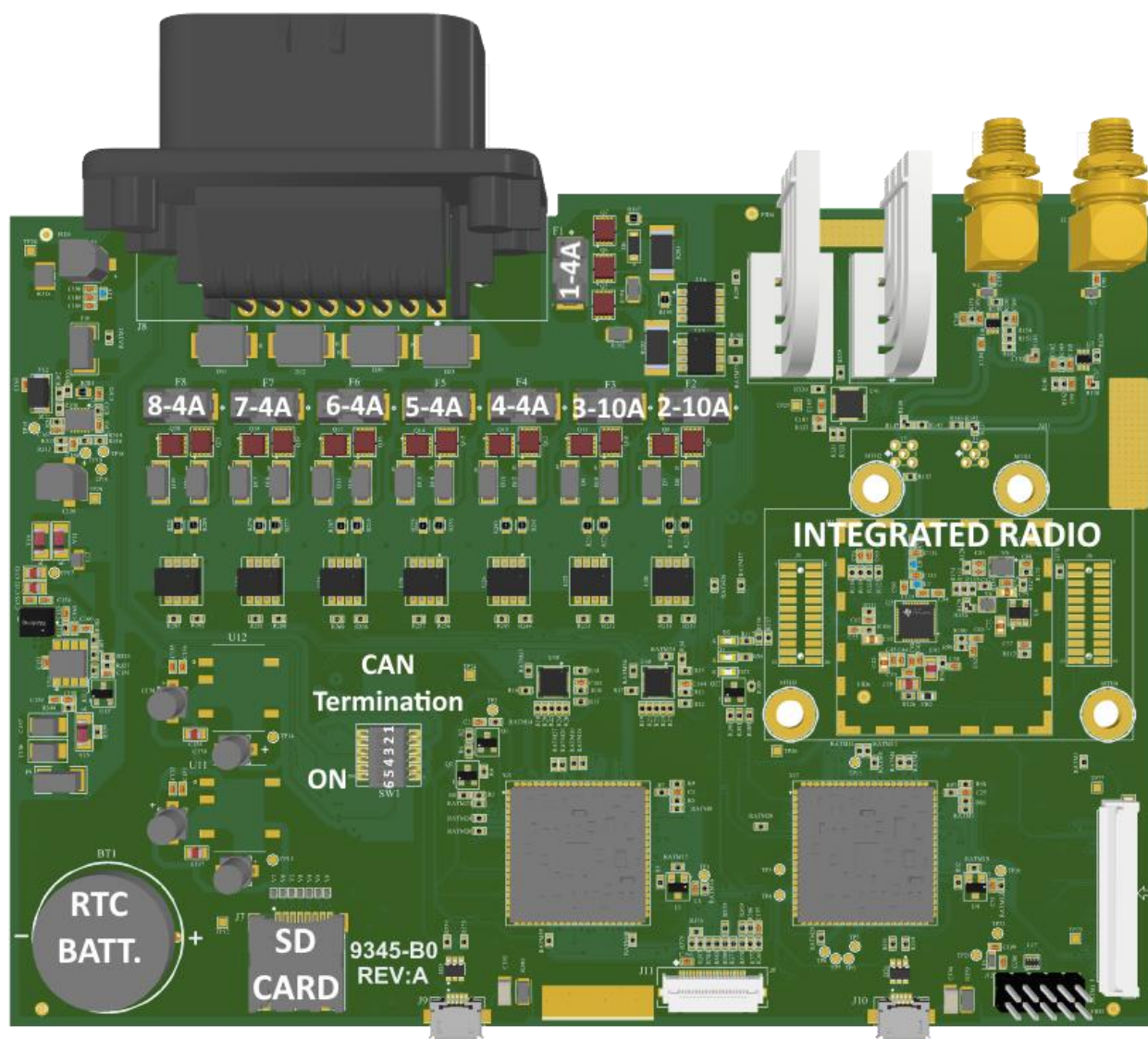
Figure 5 PCA Primary Components
