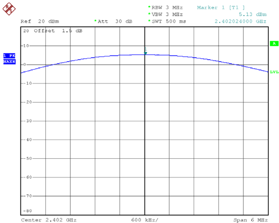
Peak Output Power Plot on Channel 00
