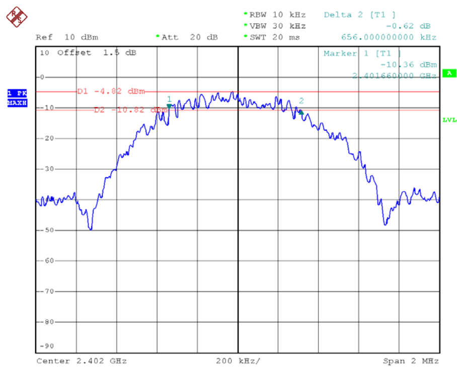
6 dB Bandwidth Plot on Channel 00
