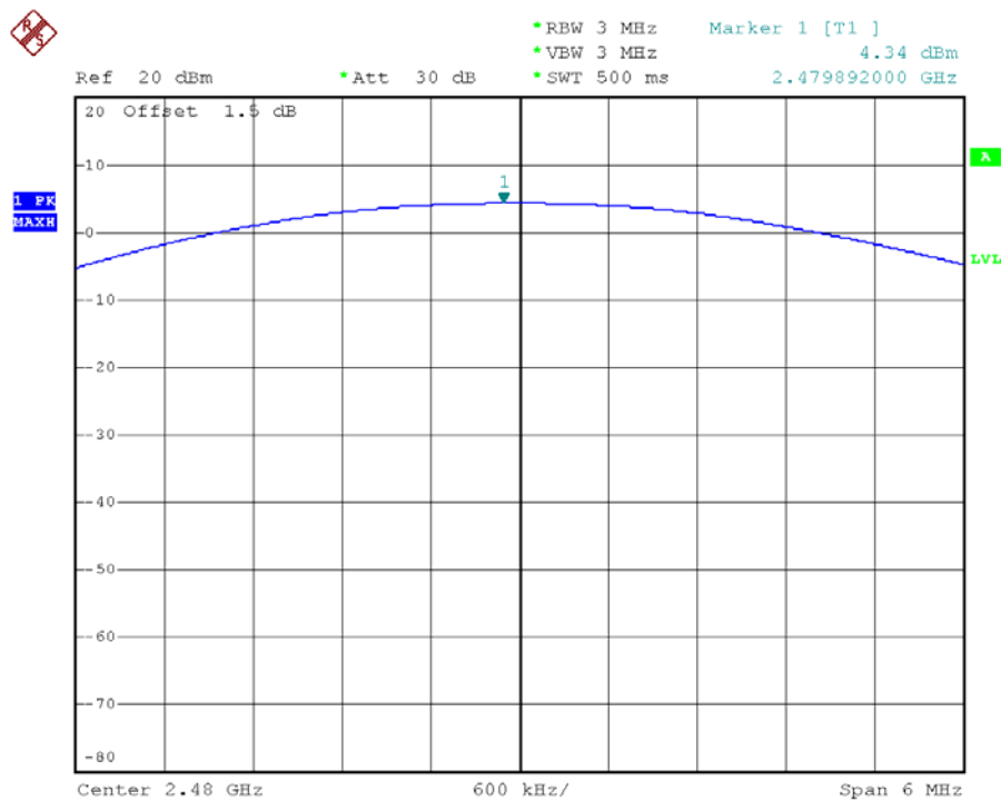
Peak Output Power Plot on Channel 39
