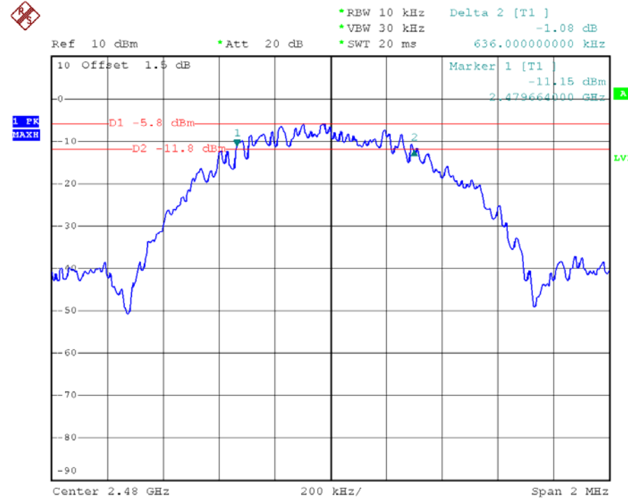
6 dB Bandwidth Plot on Channel 39
