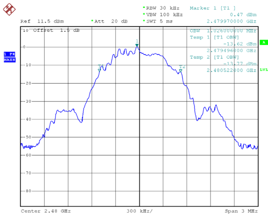
20 dB Bandwidth Plot on Channel 78
