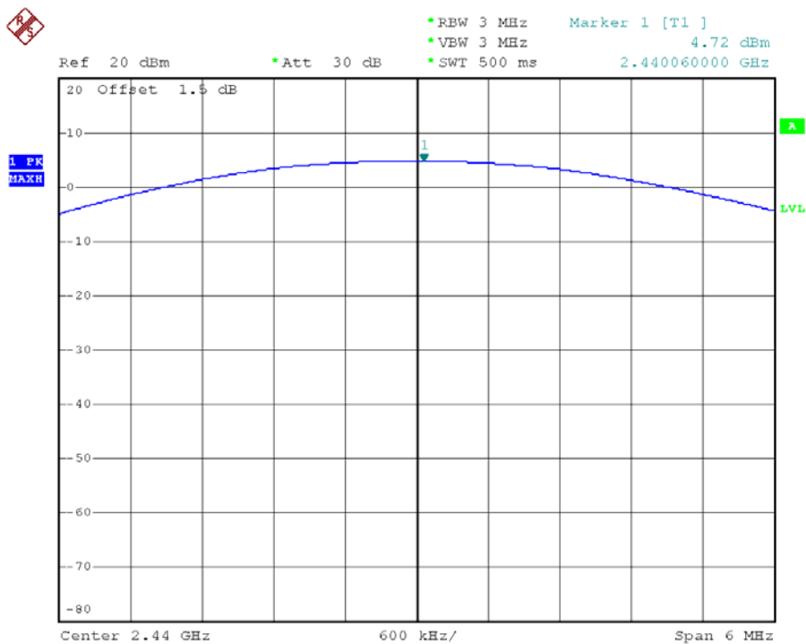
Peak Output Power Plot on Channel 19
