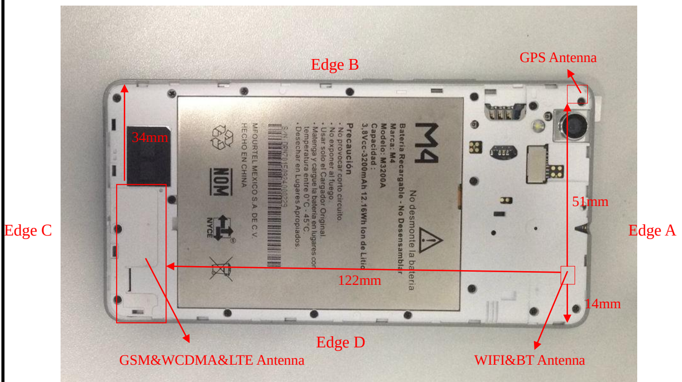
Fig. 3 Position of the antennas
