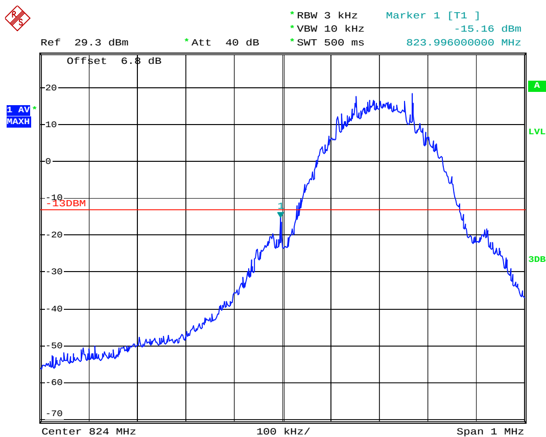
Lower Band Edge Plot on Channel 128
