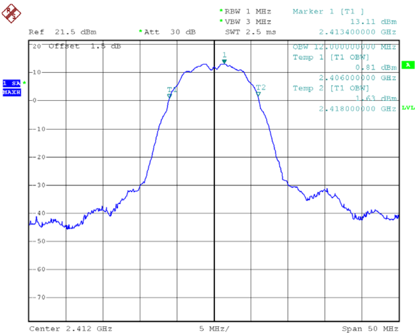
Mode 1 : 99% Occupied Bandwidth Plot on 802.11b Channel 01
