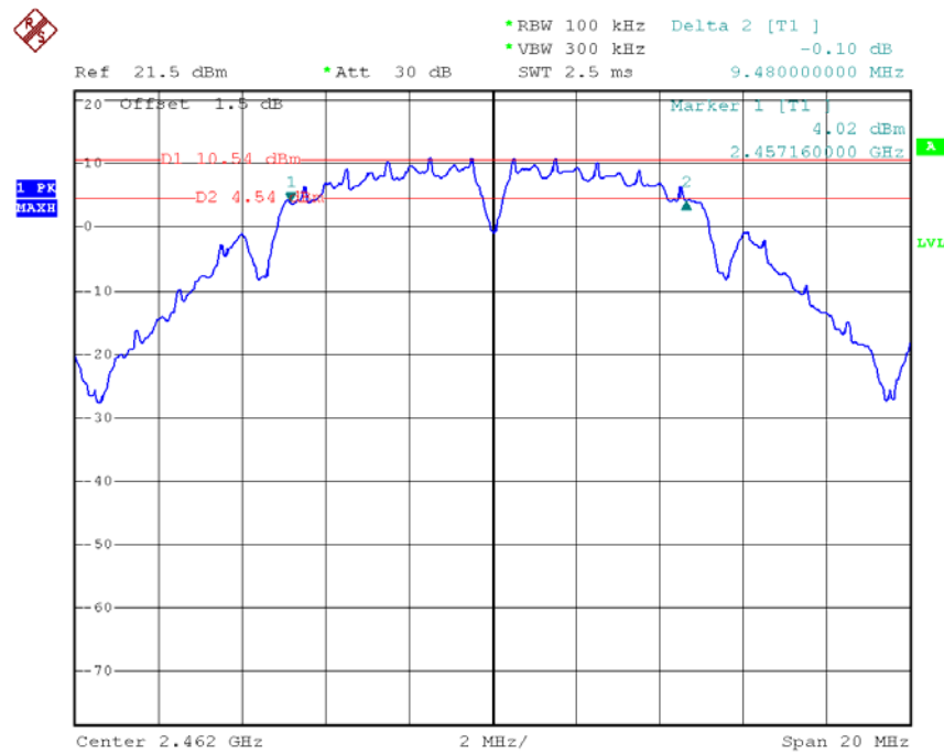
Mode 3 : 6 dB Bandwidth Plot on 802.11b Channel 11
