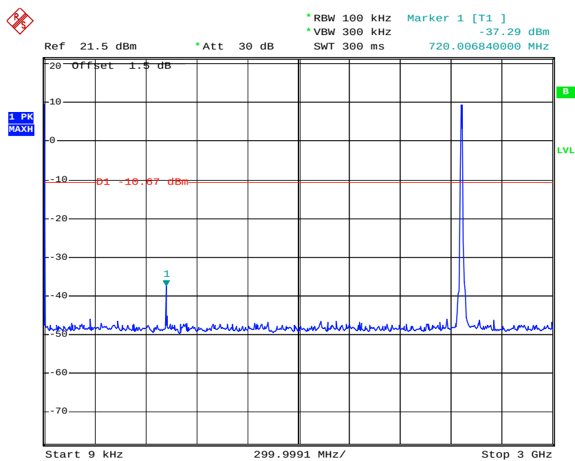
Conducted Spurious Emission Plot between 9 kHz ~ 3 GHz
