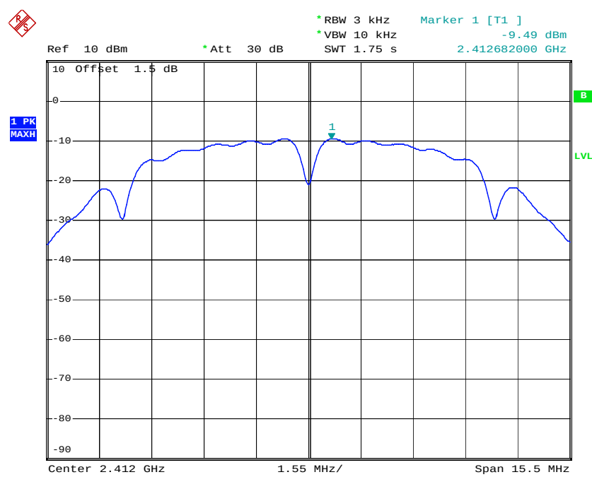
Mode 1 : PSD Plot on 802.11b Channel 01
