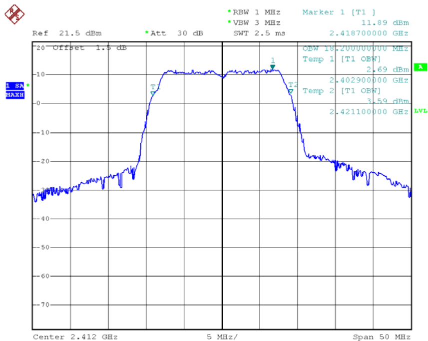
Mode 4 : 99% Occupied Bandwidth Plot on 802.11g Channel 01
