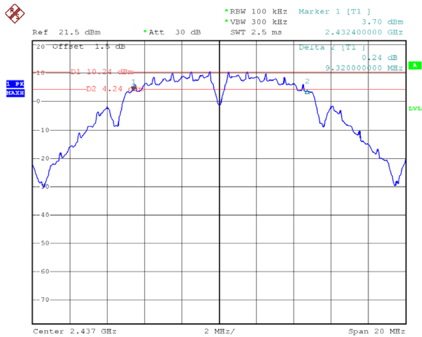
Mode 2 : 6 dB Bandwidth Plot on 802.11b Channel 06
