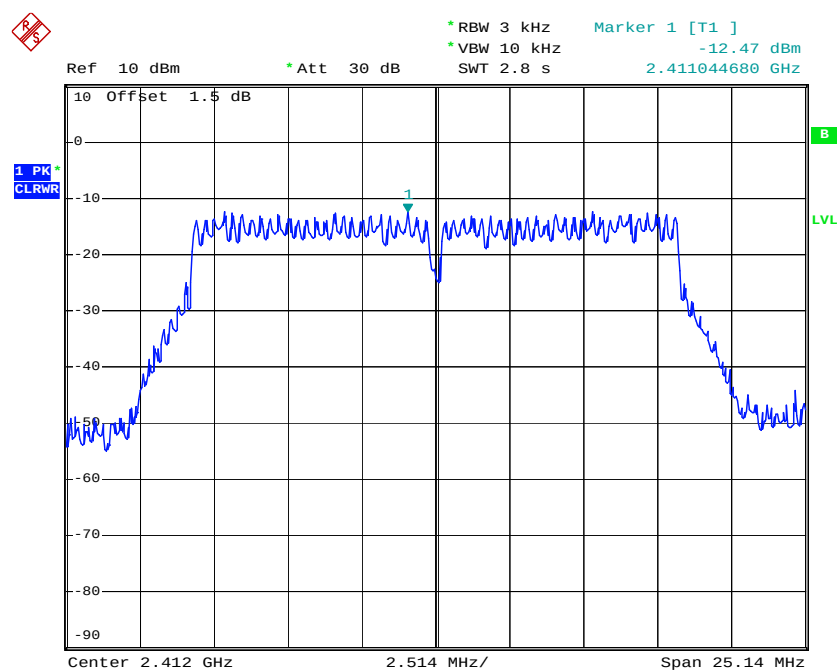
Mode 4 : PSD Plot on 802.11g Channel 01
