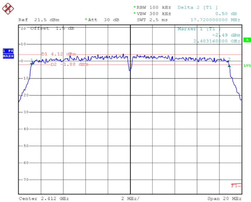
Mode 7 : 6 dB Bandwidth Plot on 802.11n Channel 01
