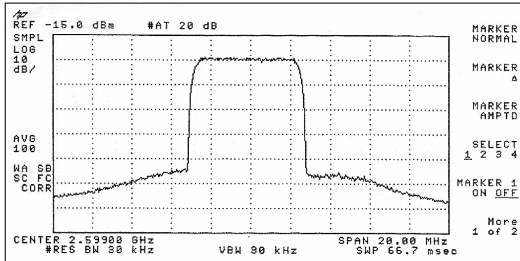
Figure 4-8. Conducted Spurious Emissions (before channel filter)
