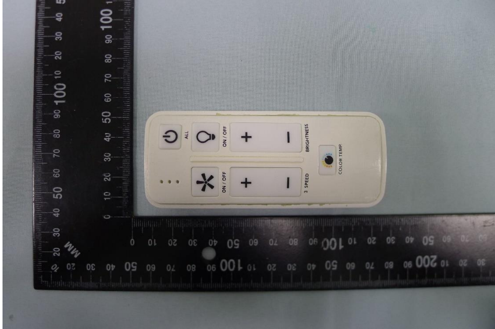
(2) EUT Photo (UC7264T3)
