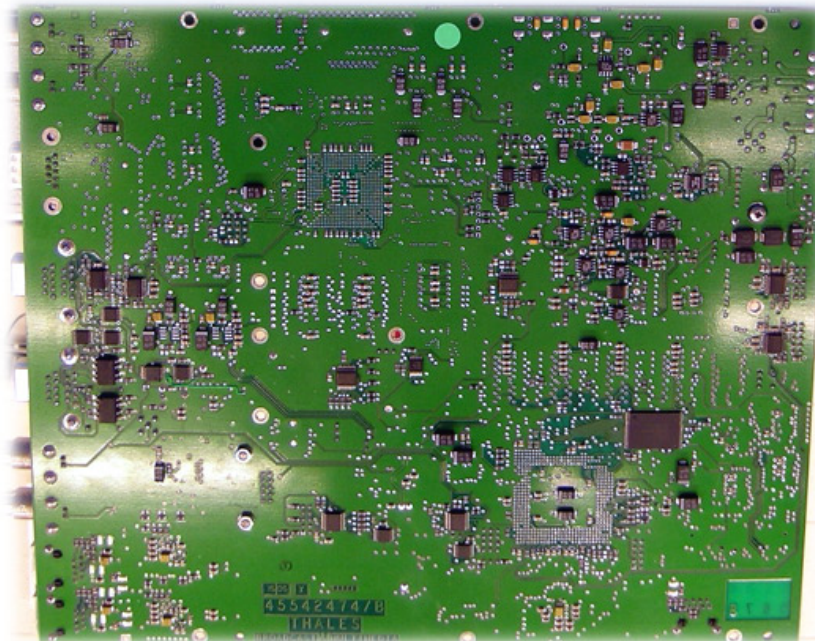
Figure 4 45324491 PCB Bottom Side View
