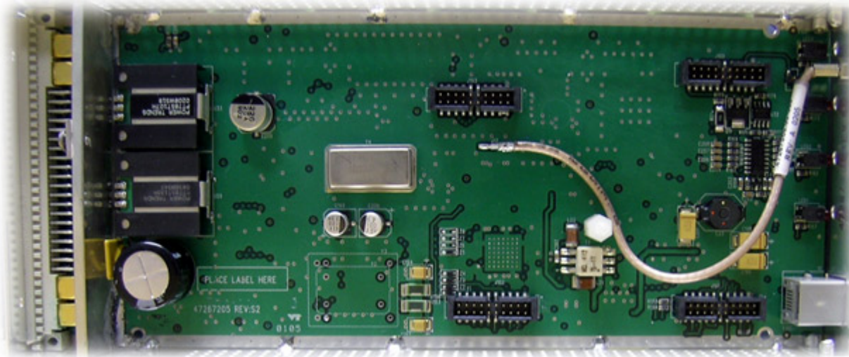
Figure 14 47267206 PCB Bottom Side View
