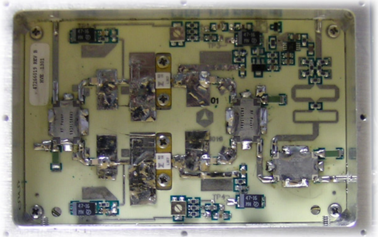
Figure 19 47267297 PCB Top Side View
