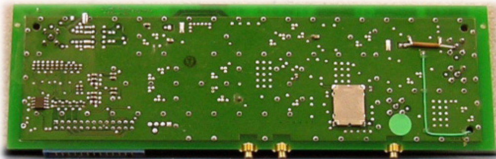
Figure 6 45324492 PCB Bottom Side View
