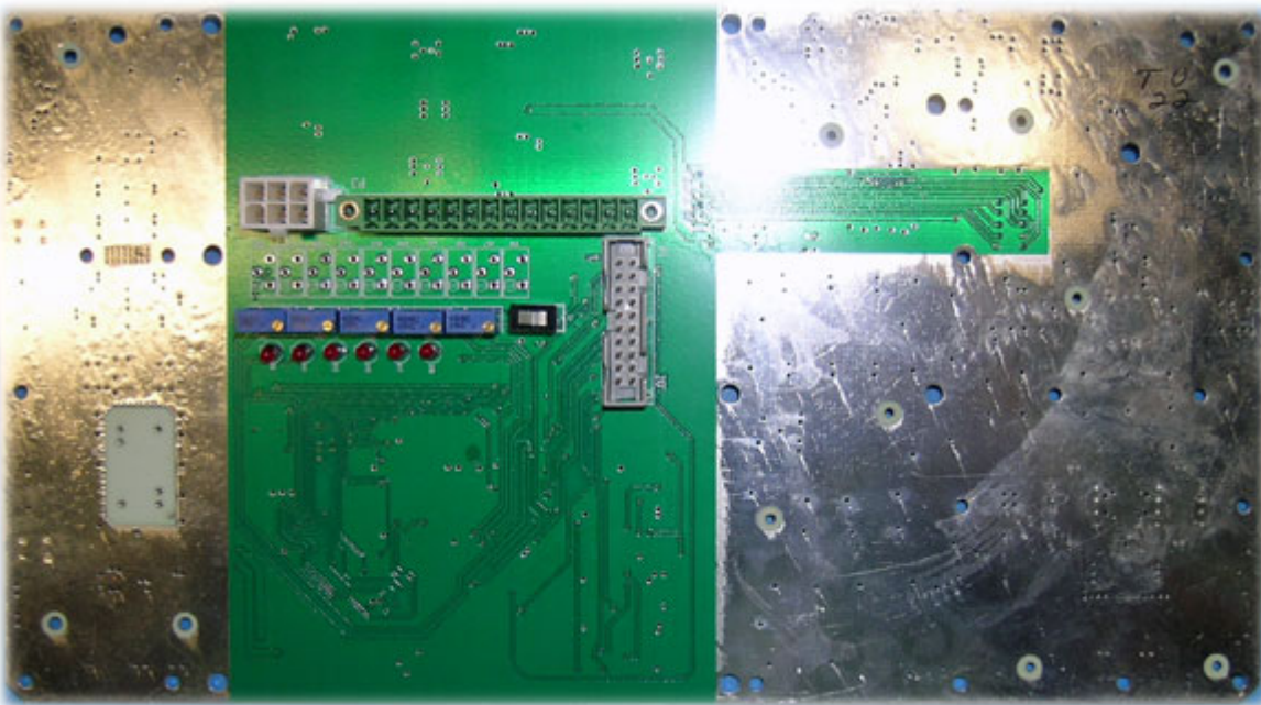
Figure 33 47267327 PCB Top Side View
