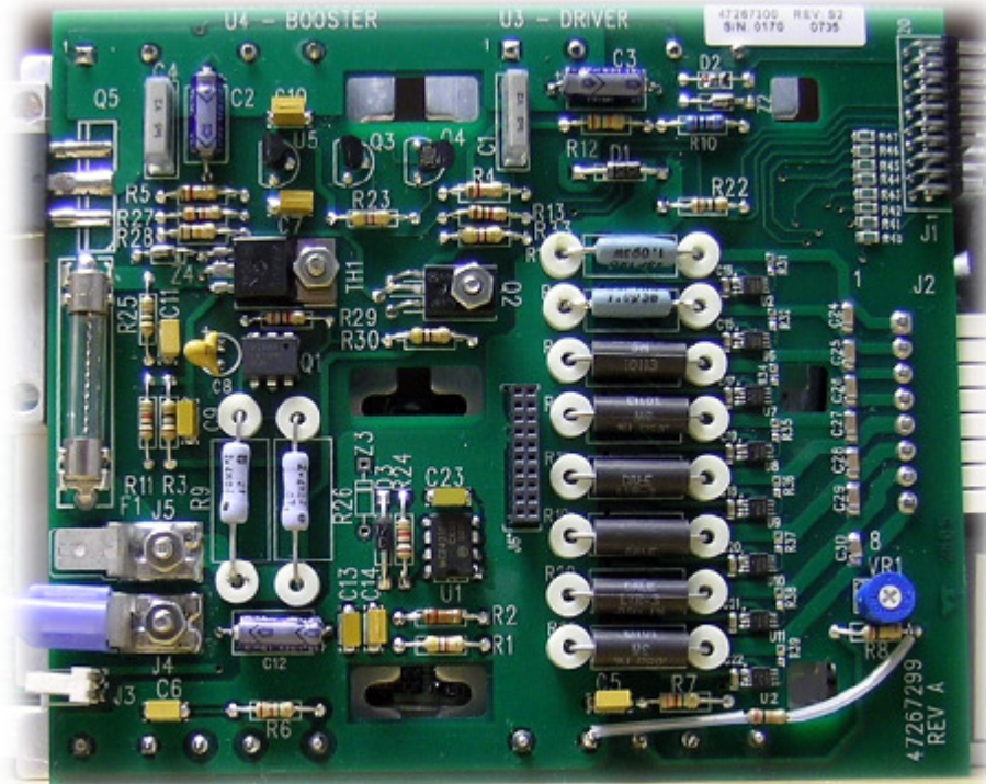
Figure 25 47267300 PCB Top Side View
