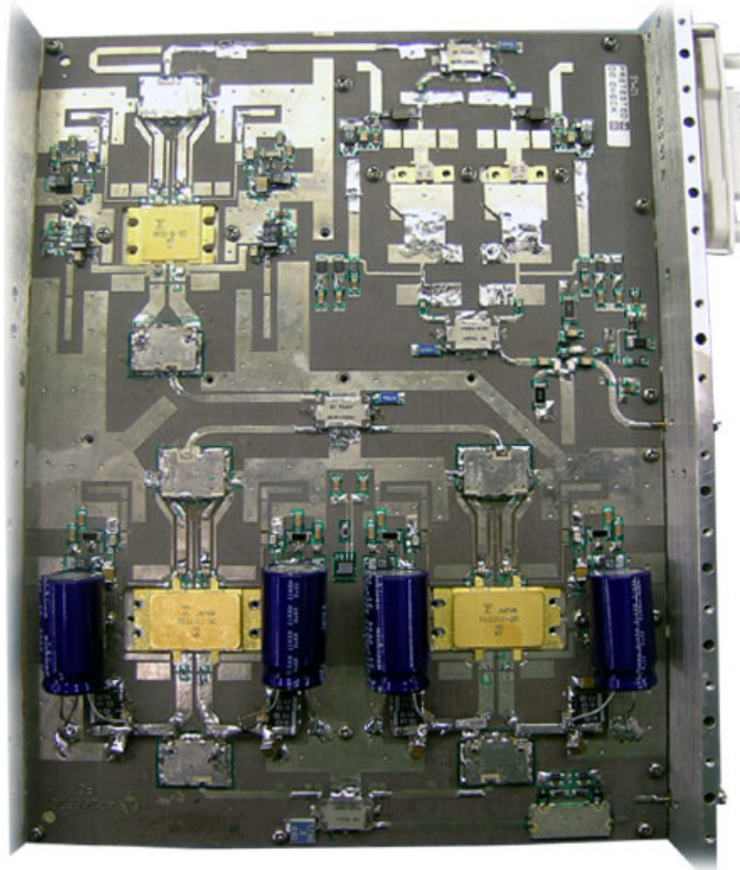
Figure 29 47267231 PCB Top Side View
