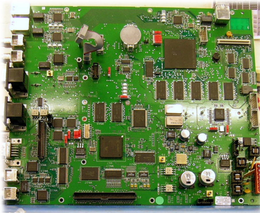
Figure 3 45324491 PCB Top Side View
