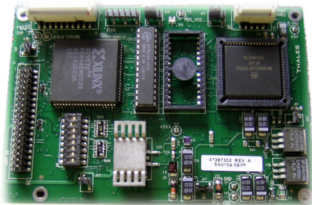
Figure 27 47267302 PCB Top Side View
