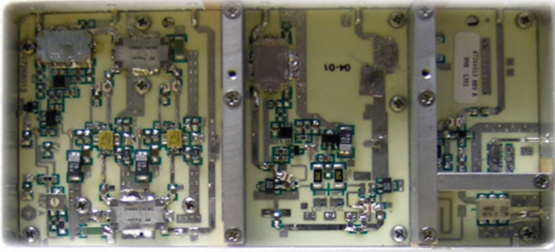
Figure 17 47267292 PCB Top Side View
