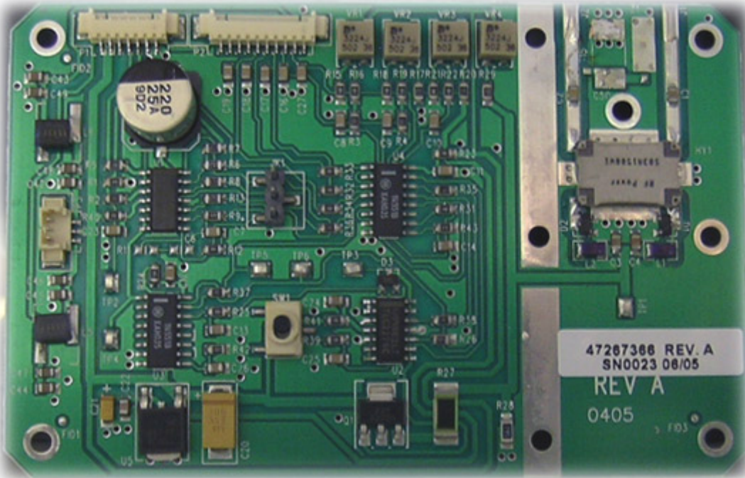
Figure 21 47267366 PCB Top Side View
