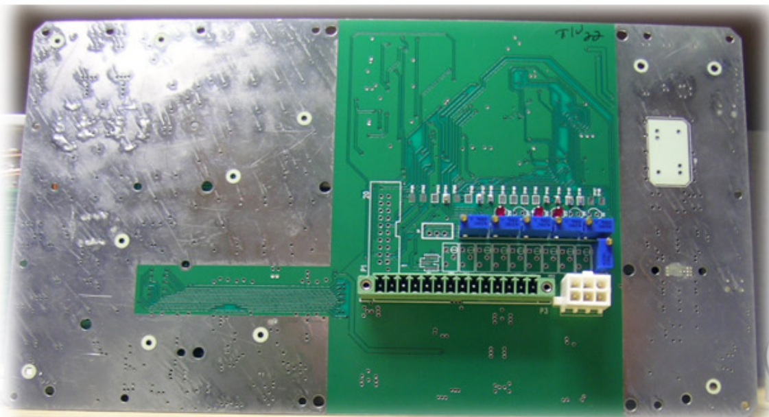
Figure 32 47267338 PCB Top Side View
