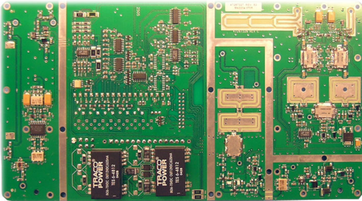
Figure 33 47267327 PCB Top Side View
