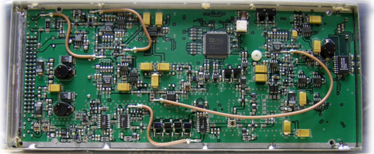
Figure 13 47267206 PCB Top Side View
