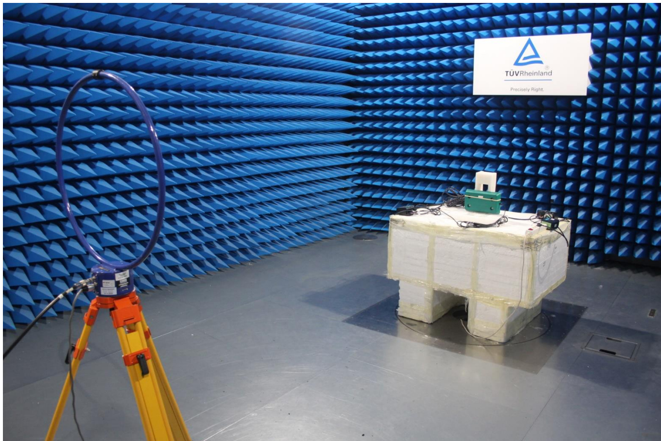
Setup EUT in Semi-AR, @3m
