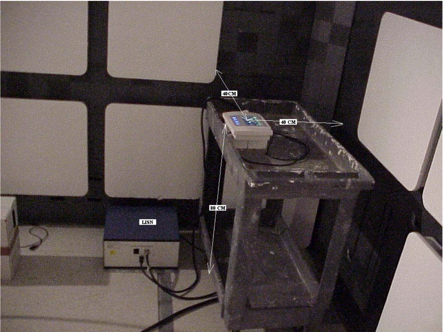
PICTURE OF ZWB LINE CONDUCTED EMISSIONS TEST ( INSIDE A LYNX TOUCH )
