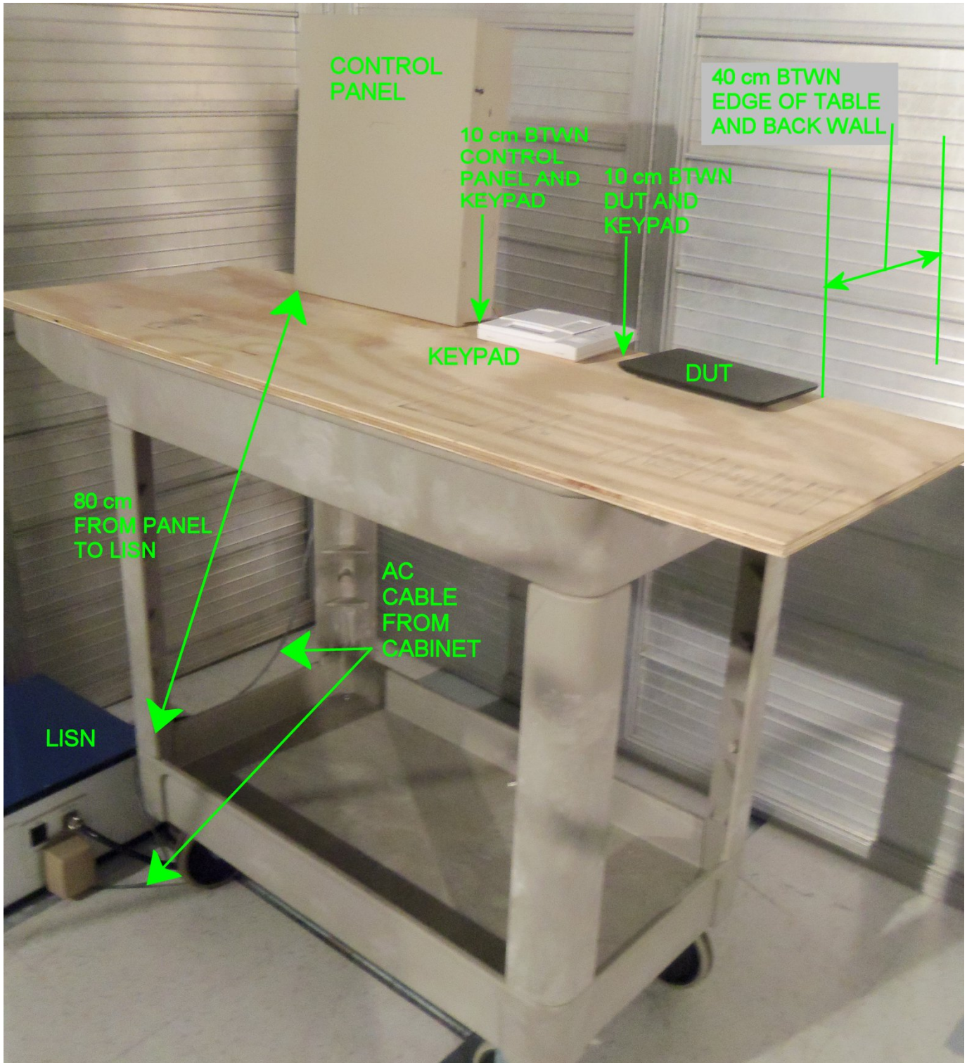
SETUP FOR TESTING
