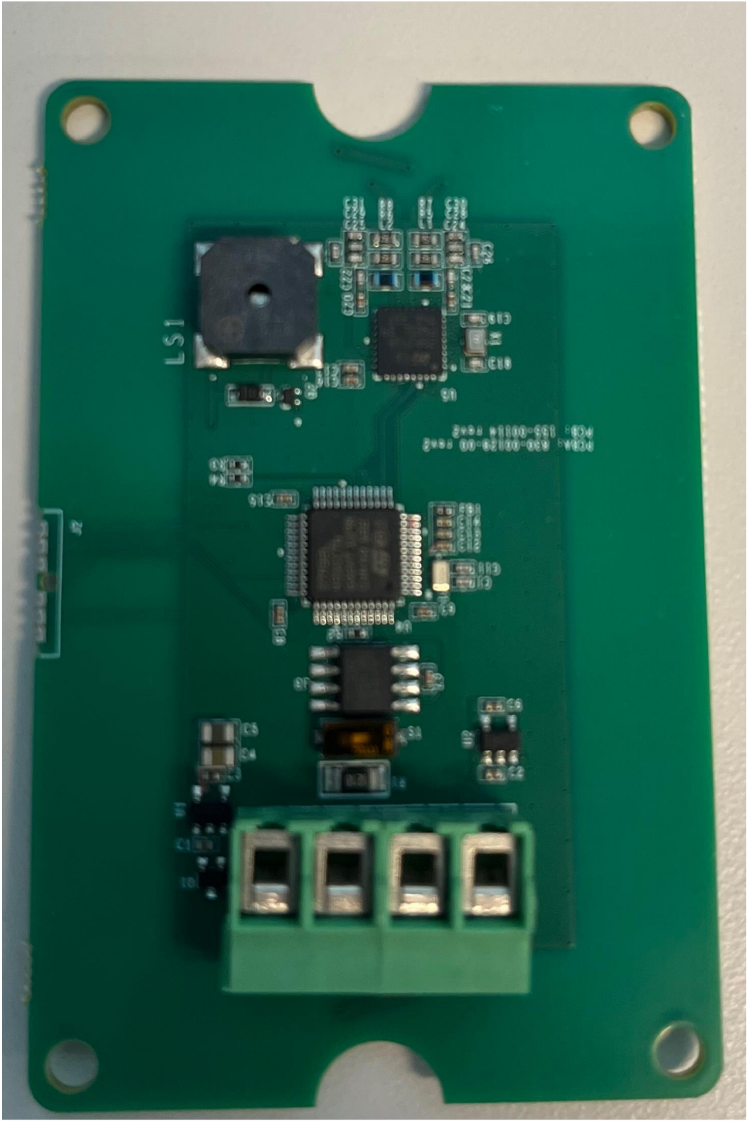
Figure 1: PCB Front
