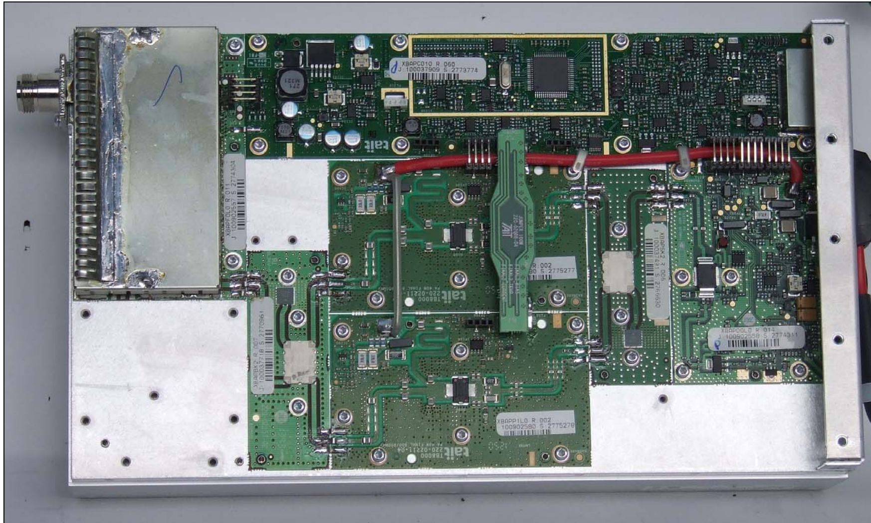
Photograph 01: 100W PA modules – Internal view
