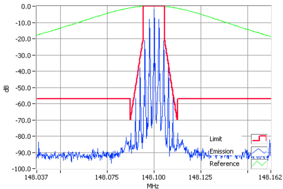
Analogue Modulation 148.1000MHz Mask D 5W RBW=100Hz, VBW=1000Hz, Detector Mode=Peak Result=Pass
