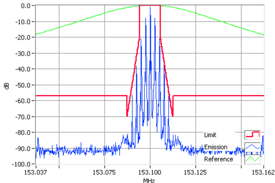
Analogue Modulation 153.1000MHz Mask D 5W RBW=100Hz, VBW=1000Hz, Detector Mode=Peak Result=Pass
