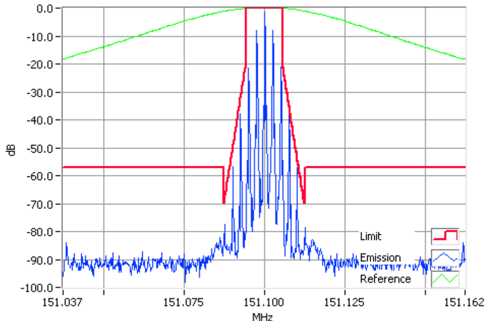
Analogue Modulation 151.1000MHz Mask D 5W RBW=100Hz, VBW=1000Hz, Detector Mode=Peak Result=Pass
