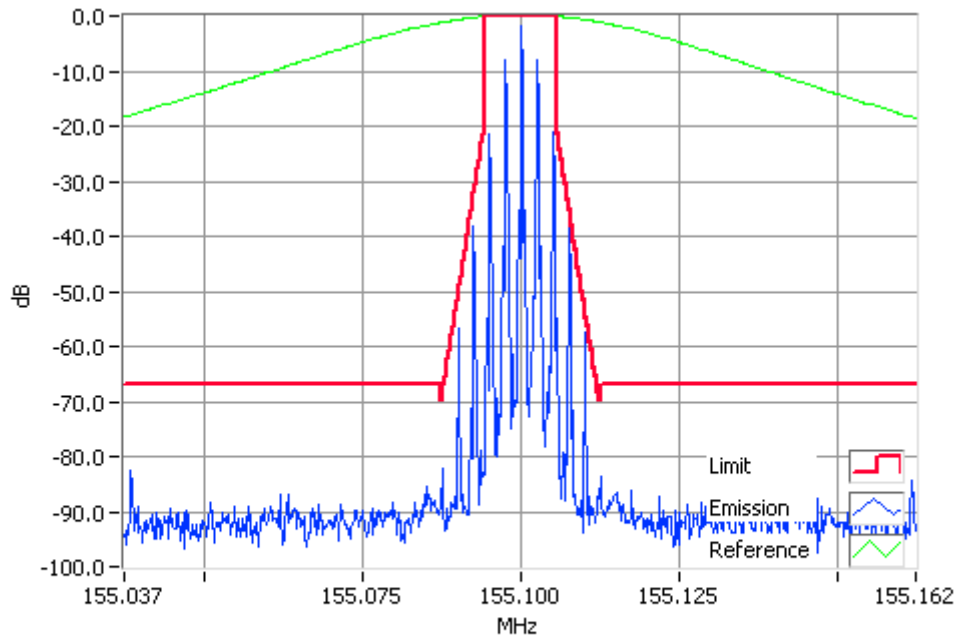
Analogue Modulation 155.1000MHz Mask D 50W RBW=100Hz, VBW=1000Hz, Detector Mode=Peak Result=Pass
