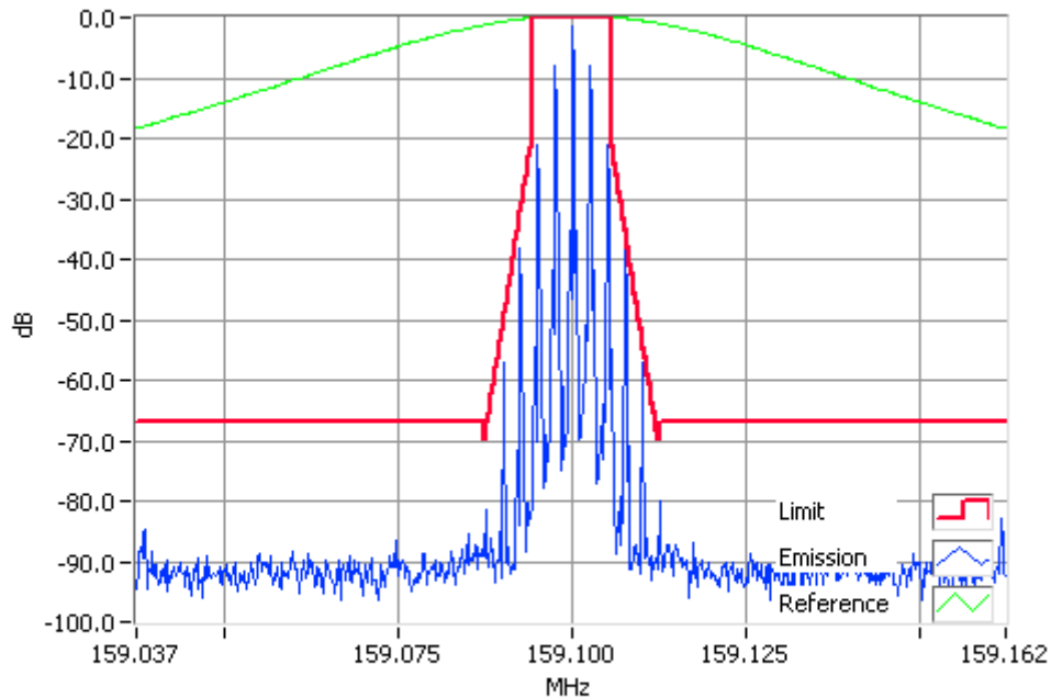
Analogue Modulation 159.1000MHz Mask D 50W RBW=100Hz, VBW=1000Hz, Detector Mode=Peak Result=Pass
