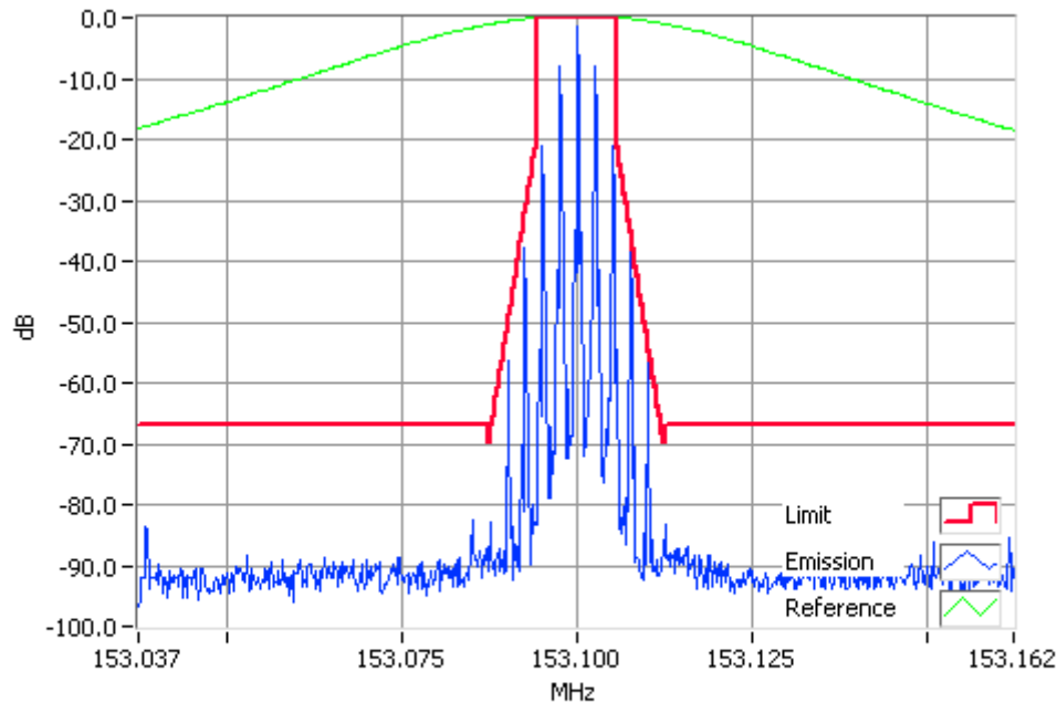
Analogue Modulation 153.1000MHz Mask D 50W RBW=100Hz, VBW=1000Hz, Detector Mode=Peak Result=Pass
