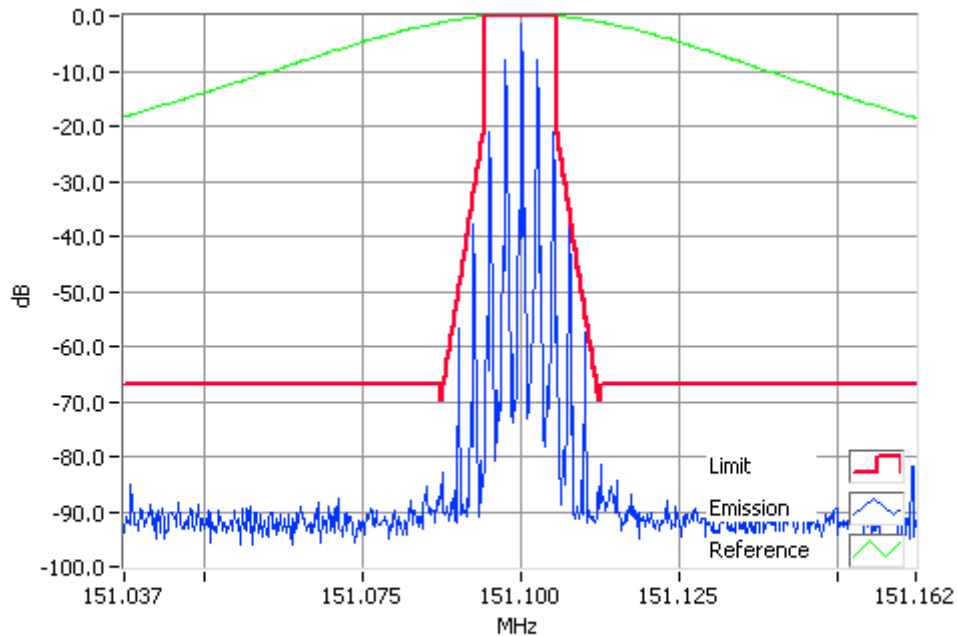
Analogue Modulation 151.1000MHz Mask D 50W RBW=100Hz, VBW=1000Hz, Detector Mode=Peak Result=Pass
