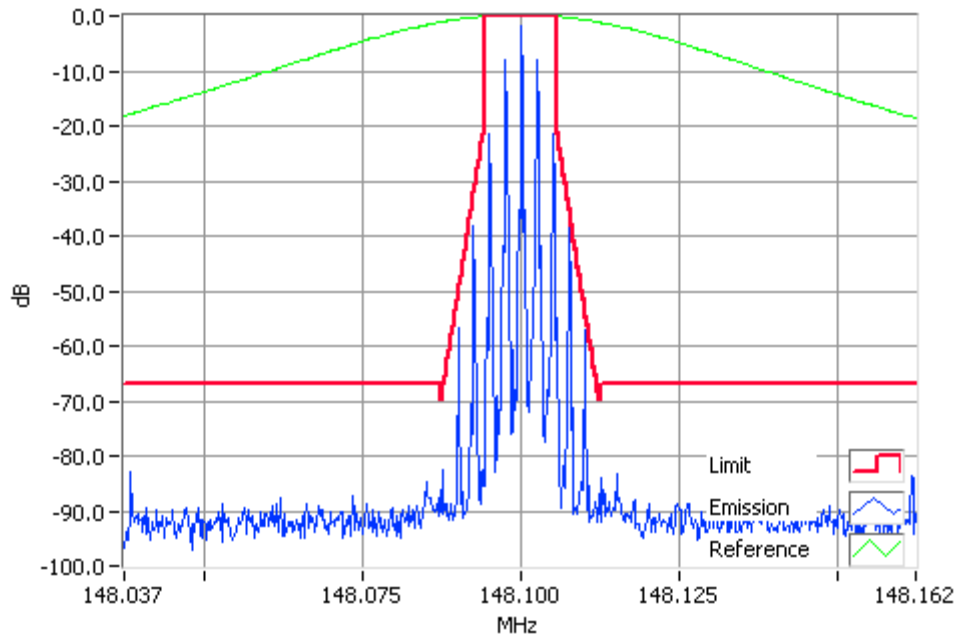
Analogue Modulation 148.1000MHz Mask D 50W RBW=100Hz, VBW=1000Hz, Detector Mode=Peak Result=Pass
