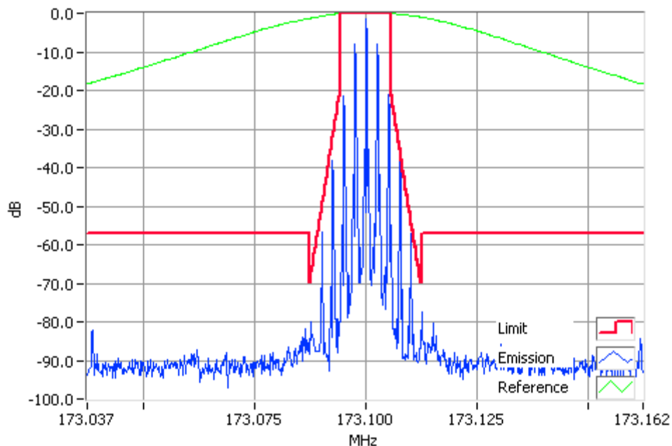
Analogue Modulation 173.1000MHz Mask D 5W RBW=100Hz, VBW=1000Hz, Detector Mode=Peak Result=Pass
