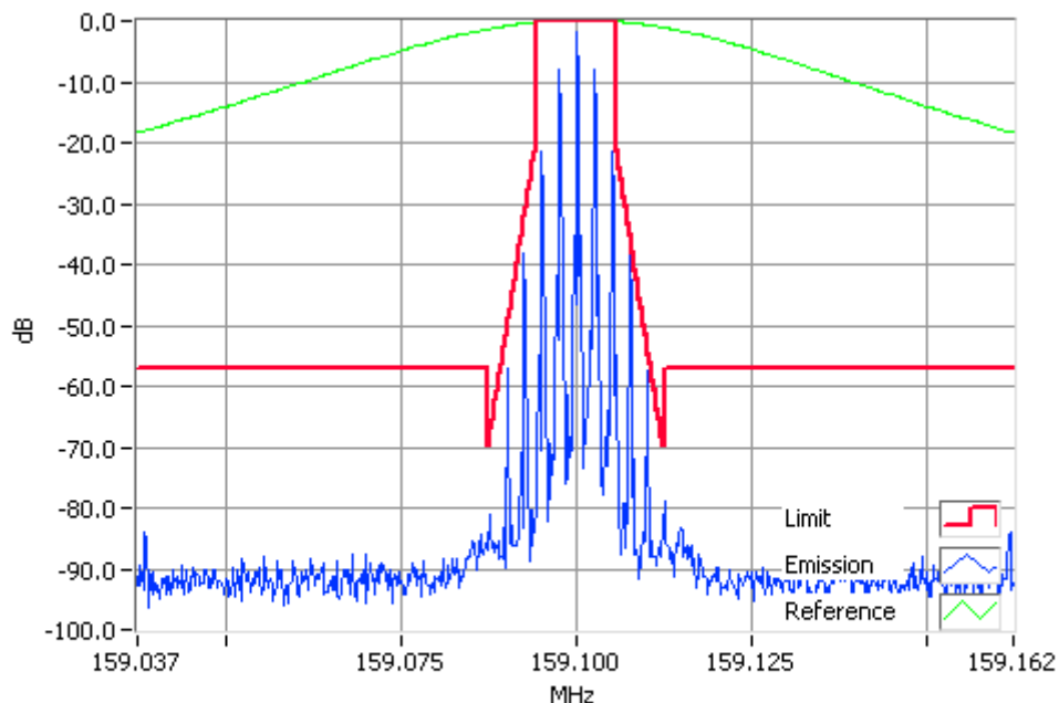
Analogue Modulation 159.1000MHz Mask D 5W RBW=100Hz, VBW=1000Hz, Detector Mode=Peak Result=Pass
