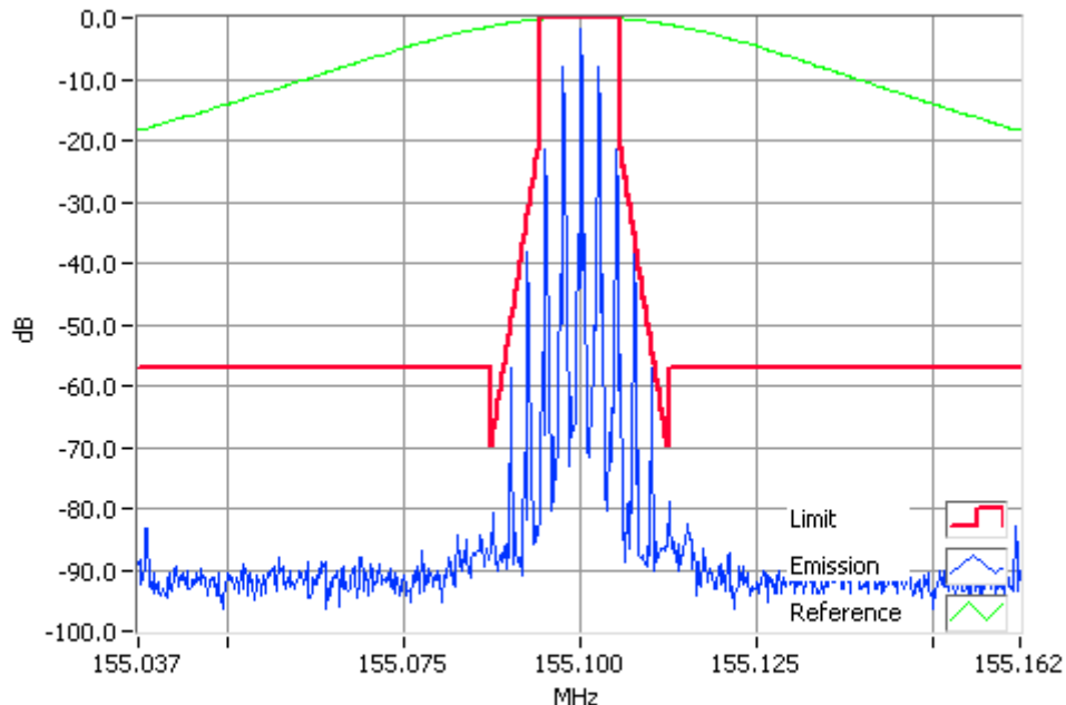
Analogue Modulation 155.1000MHz Mask D 5W RBW=100Hz, VBW=1000Hz, Detector Mode=Peak Result=Pass
