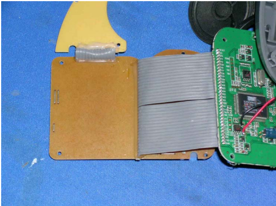
Base Unit Display rear side (View 1)
