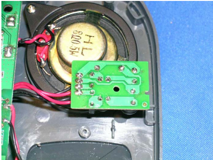
Base Unit DSL filter rear side
