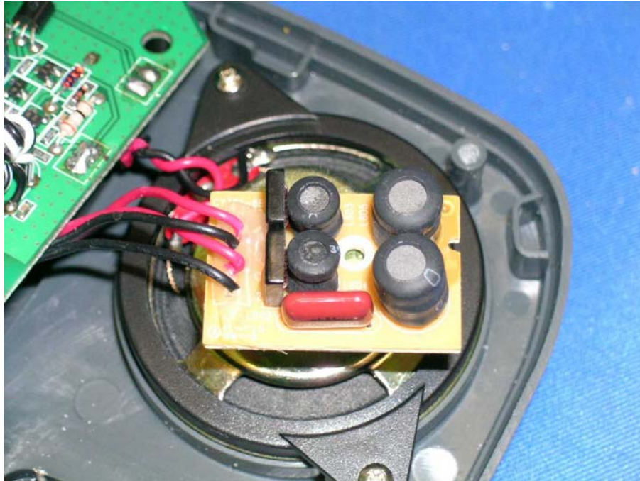
Base Unit DSL filter front side
