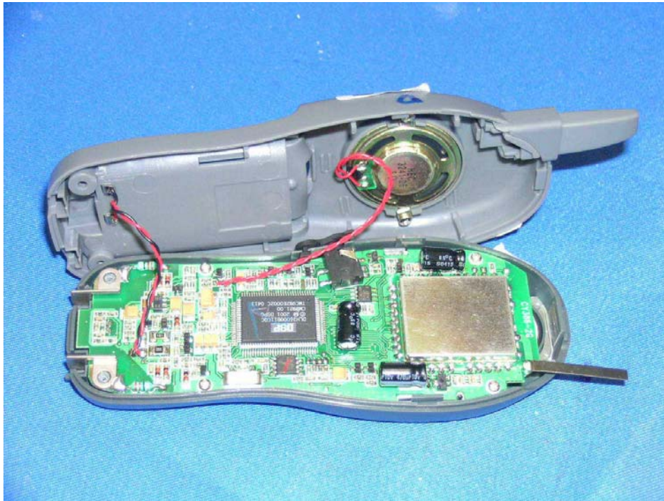
Handset assembly
