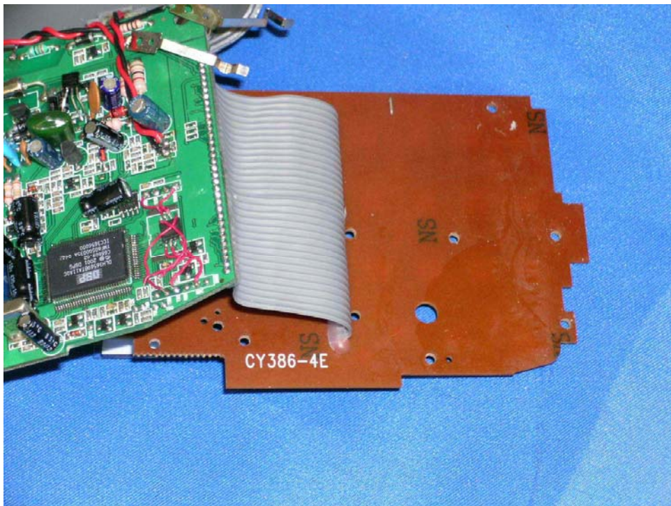
Base Display Board rear side (View 1)
