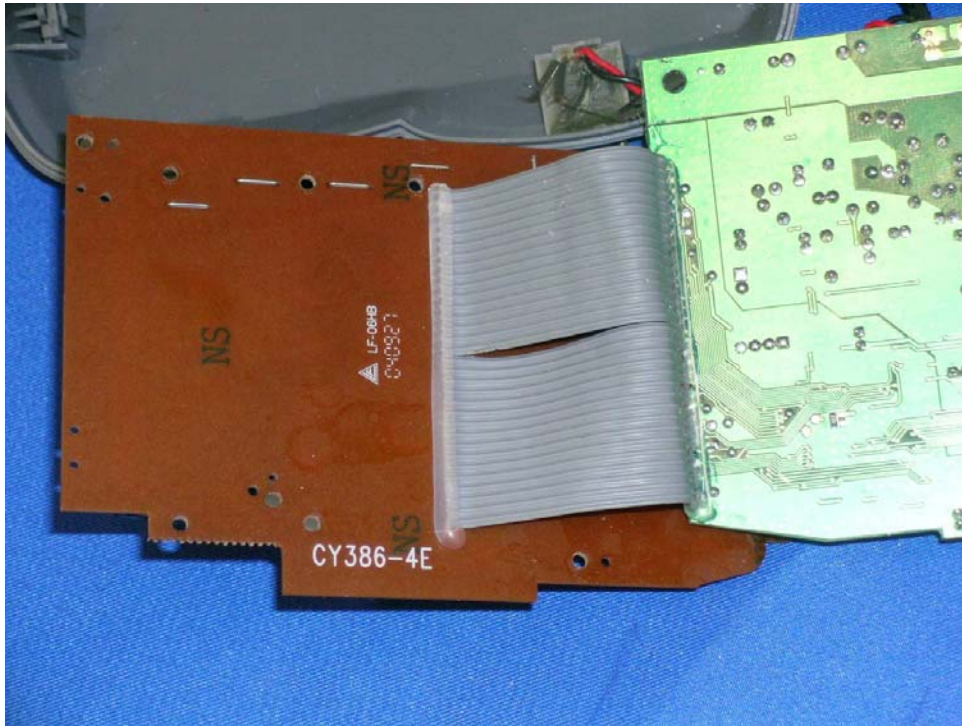
Base Display Board rear side (View 2)
