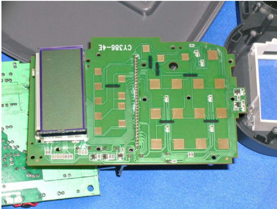
Base Display Board front side
