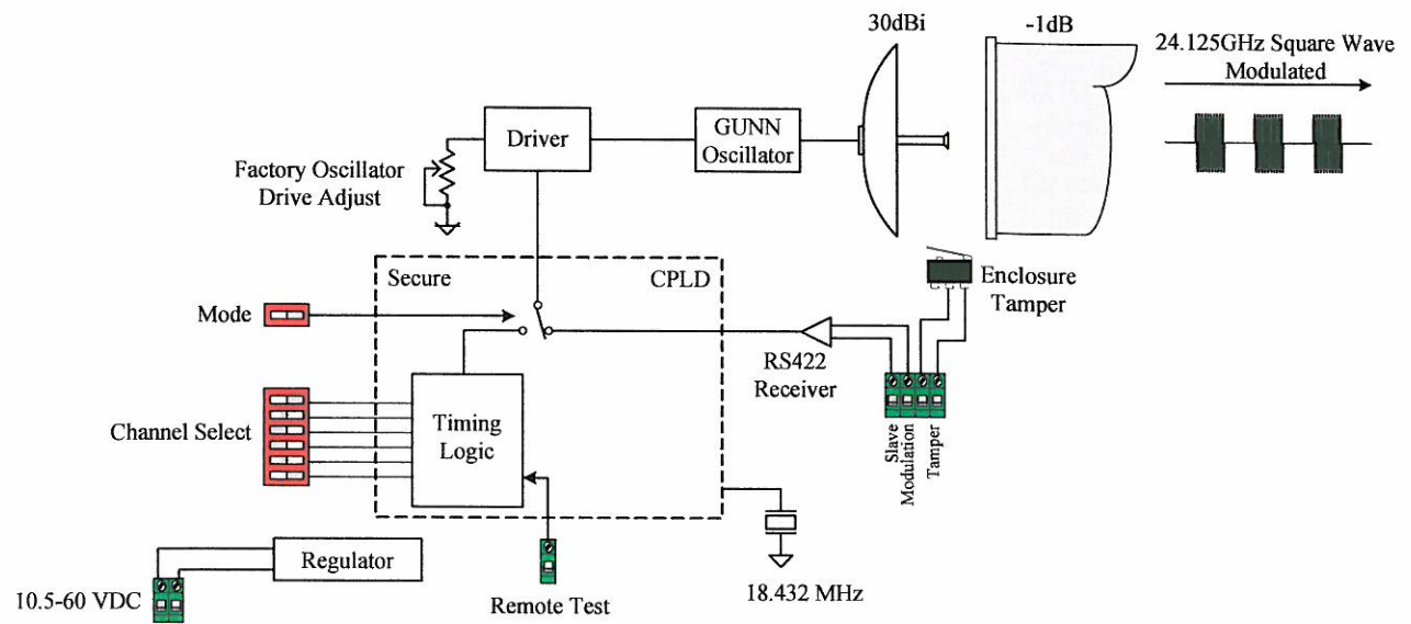
Model 330 Transmitter Block Diagram
