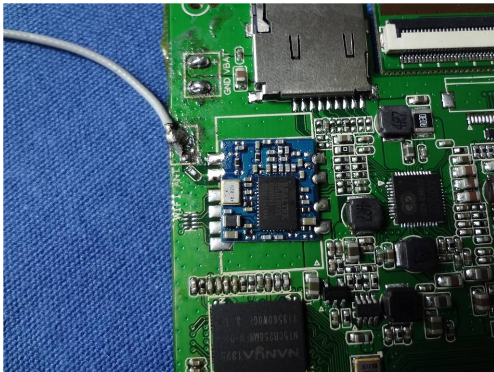
PHOTO OF RF MODUEL
