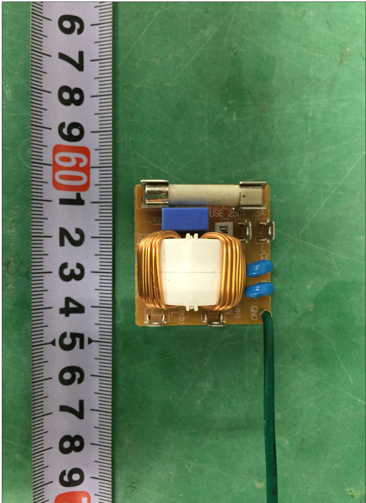
► Front View of Line Filter
