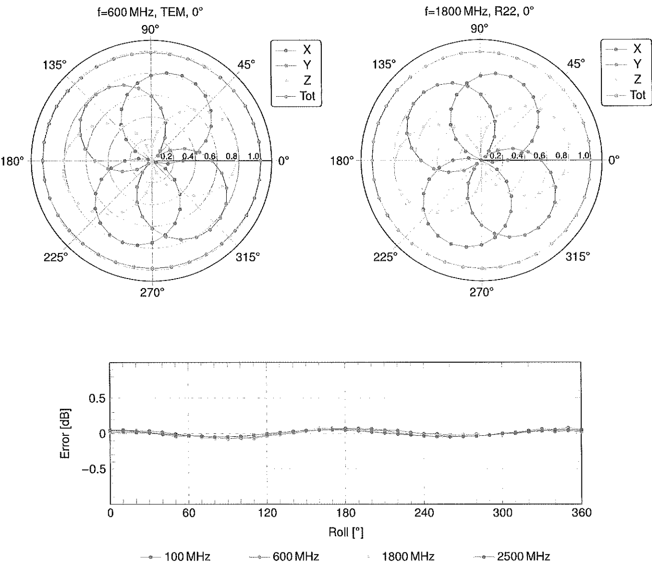
Uncertainty of Axial Isotropy Assessment: \pm 0.5\% ( k=2 )
