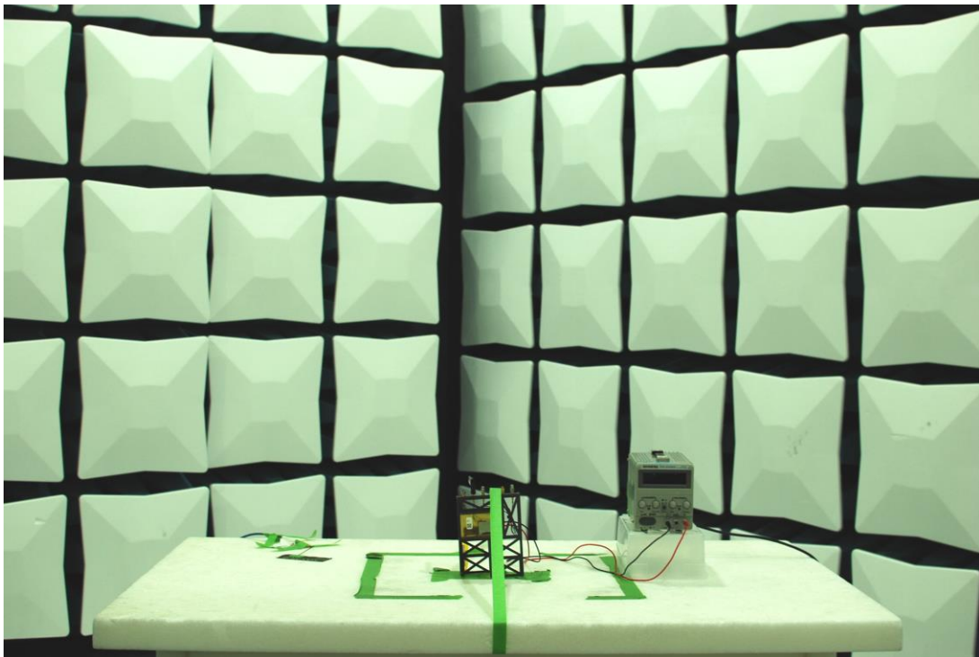
Figure 6. Test Setup – Z Position – 30MHz-1GHz
