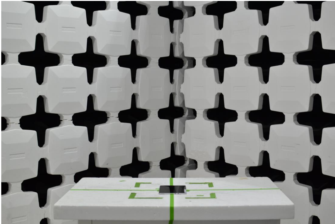
Figure 1. Test Setup – X Position – 30MHz-1GHz – Pen Charging
