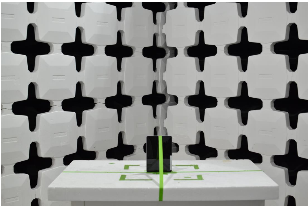
Figure 2. Test Setup – Y Position – 30MHz-1GHz – Pen Charging
