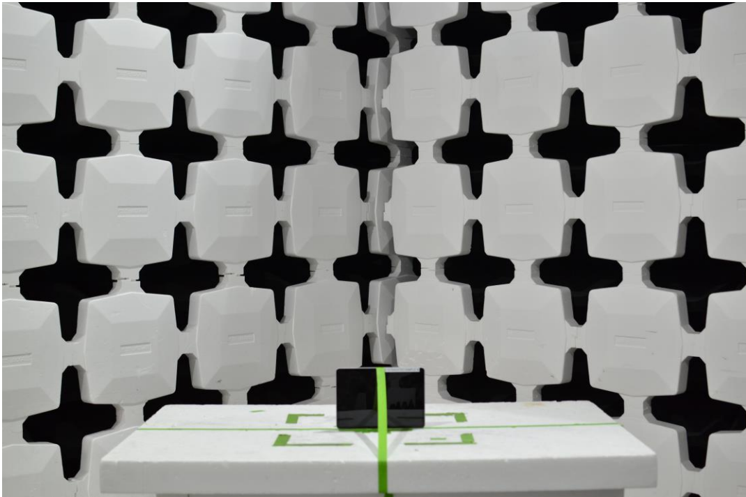
Figure 3. Test Setup – Z Position – 30MHz-1GHz – Pen Charging
