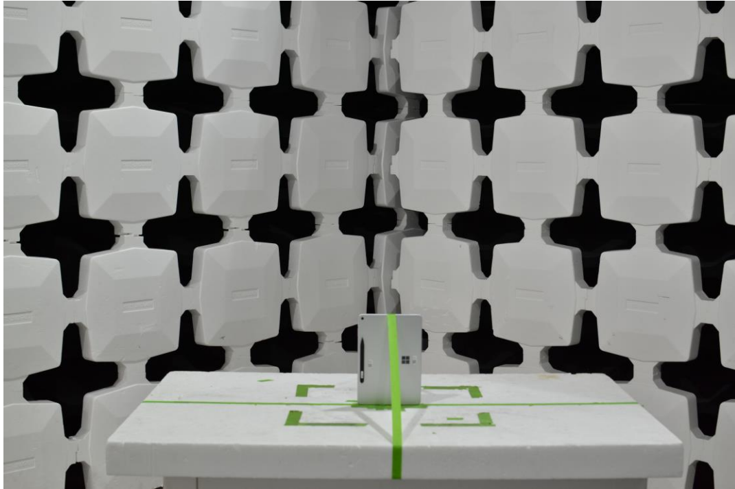
Figure 5. Test Setup – Y Position – 30MHz-1GHz – Pen Charging
