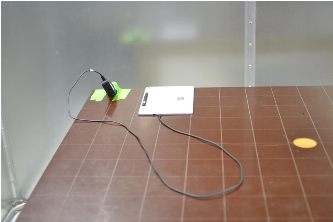
Figure 8. Test Setup – ACLC – <30MHz – Pen Charging
