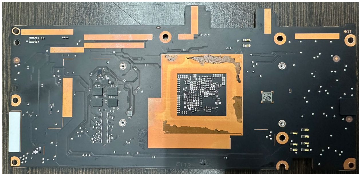
Figure 3: PCB Bottom side with covers removed
